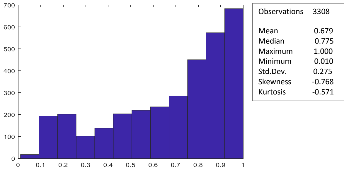
Figure 1. Histogram and descriptive statistics for the adjusted health state valuations
