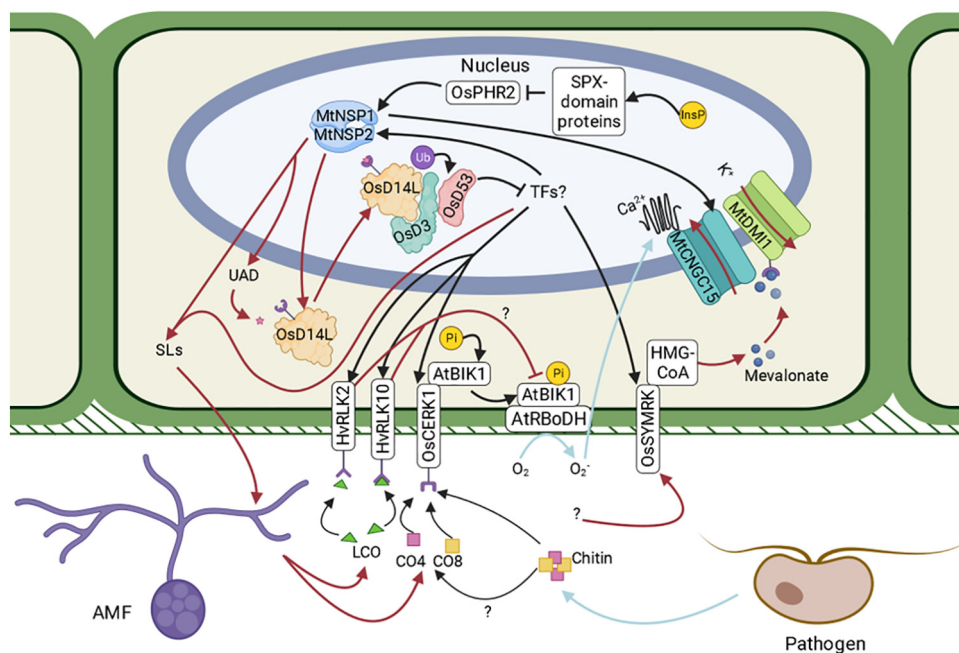
Figure 2. The release of arbuscular mycorrhizal (AM) fungi-recruiting strigolactones (SLs) and the detection of AM fungi are regulated by the phosphate starvation response. Inorganic phosphate ( P_i ) becomes incorporated into inositol phosphate (InsP), which can bind to SPX domain proteins and enables their repression of PHR2 in rice [46,92]. Under low inorganic phosphate abundance, PHR2 is active and promotes the transcription of NSP1 and NSP2 in Medicago truncatula [42]. The activity of NSP1 and NSP2 in rice promotes the biosynthesis of strigolactones, which are then exported to the rhizosphere where they have stimulatory effects on AM fungi [37,38,93]. The production of SLs likely also causes the production of an unidentified apocarotenoid derivative (UAD), which acts as a ligand to rice D14L, enabling it to form a Skp, Cullin, F-box (SCF) complex with D3 [43,52]. The D14L–D3 SCF complex ubiquitinates the transcriptional repressor D53/AtSMAX1 and targets it for proteasomal degradation [52,94–96]. The degradation of D53 or its orthologues causes many cell surface receptors to become upregulated, including CERK1 and SYMRK in rice [43]. The recognition of chitinous elicitors by CERK1 results in the phosphorylation of associated cytosolic protein kinases, leading to transphosphorylation and activation of NADPH oxidases, which release a reactive oxygen species (ROS) burst [68]. In Medicago , the binding of lipochitooligosaccharide (LCO) to Nod Factor Perception (NFP; the orthologue to HvRLK2 and HvRLK10) can prevent chitooligosaccharide (CO)-dependent ROS production via an unidentified mechanism [53]. In pathogen interactions, a ROS burst can induce nuclear calcium oscillations via an unknown mechanism [97]. Nuclear calcium oscillations are also induced during AM symbiosis, where mevalonate acts as a secondary messenger released after recognition of the AM fungus and binds to MtDMI1 to activate an efflux of potassium ions from the nucleus, which sustains an influx of calcium ions via the coupled channel protein MtCNGC15 [51]. Predominantly symbiosis-specific processes are shown in red, while predominantly immunity-driven processes are shown in blue, and shared processes are in black; Abbreviations: AM, arbuscular mycorrhizal; TFs, transcription factors; Ub, ubiquitin.
