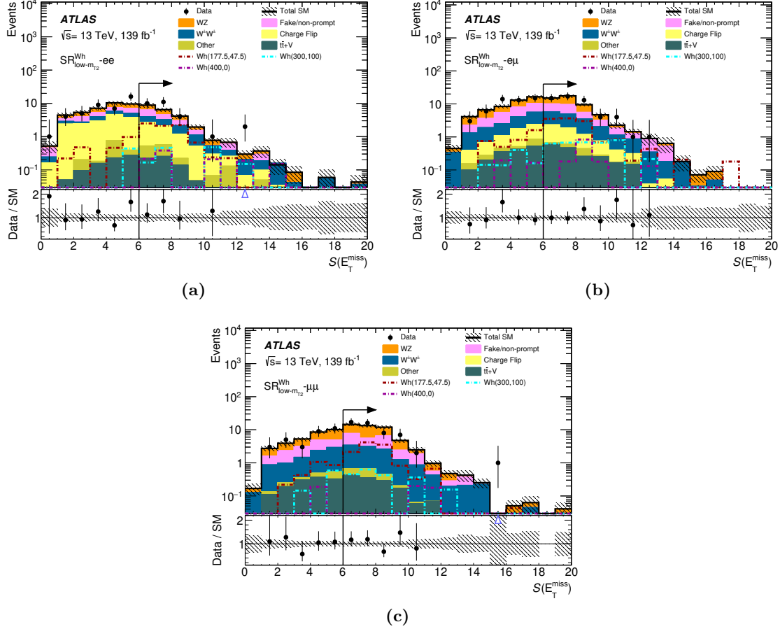
Figure 9. S(E_T^{\text{miss}}) distributions after the background-only fit, showing the data and the post-fit expected background in all the flavour bins of the SR_{\text{low-}m_{T2}}^{Wh} region. The vertical black line and the corresponding arrow indicates the cut defining the SR_{\text{low-}m_{T2}}^{Wh} region. The last bin includes overflow. The ‘Other’ category contains the t\bar{t}+H , rare top, triboson, and other diboson processes with the SS final state. Distributions for three representative signal mass points of the Wh model are overlaid. The bottom panel shows the ratio of the observed data to the predicted yields. The hatched bands indicate the combined theoretical, experimental, data-driven and MC statistical uncertainties.
