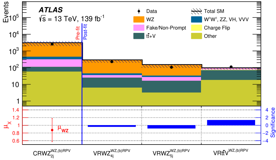
Figure 4. Expected SM backgrounds and data yields in \text{CRWZ}_{2j}^{WZ,(b)RPV} , \text{VRWZ}_{4j}^{WZ,(b)RPV} , \text{VRWZ}_{5j}^{WZ,(b)RPV} and \text{VRt}\bar{t}V^{WZ,(b)RPV} designed for the WZ model and models of higgsino-like electroweakinos in RPV SUSY. The ‘Other’ category contains the t\bar{t}+H and rare top processes with the SS final state. The error band includes the statistical, theoretical and experimental uncertainties. The bottom panel shows the scale factor obtained from \text{CRWZ}_{2j}^{WZ,(b)RPV} ( \mu_{WZ} ) and the statistical significance [204] of the discrepancy between the observed number of events and the SM expectation.
