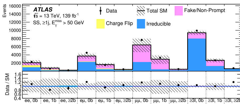
Figure 5. Data event yields compared with the expected contributions from the irreducible and the reducible backgrounds after a loose preselection requiring SS leptons, E_T^{\text{miss}} > 50 GeV and at least one jet with p_T > 25 GeV. The observed and predicted event yields are classified as a function of the number of leptons and their flavour, as well as the number of b -jets. The error bars only include the statistical uncertainty and the full uncertainties for the data-driven background estimates, in order to validate the matrix method itself. The bottom panel shows the ratio of the observed data to the predicted yields.
