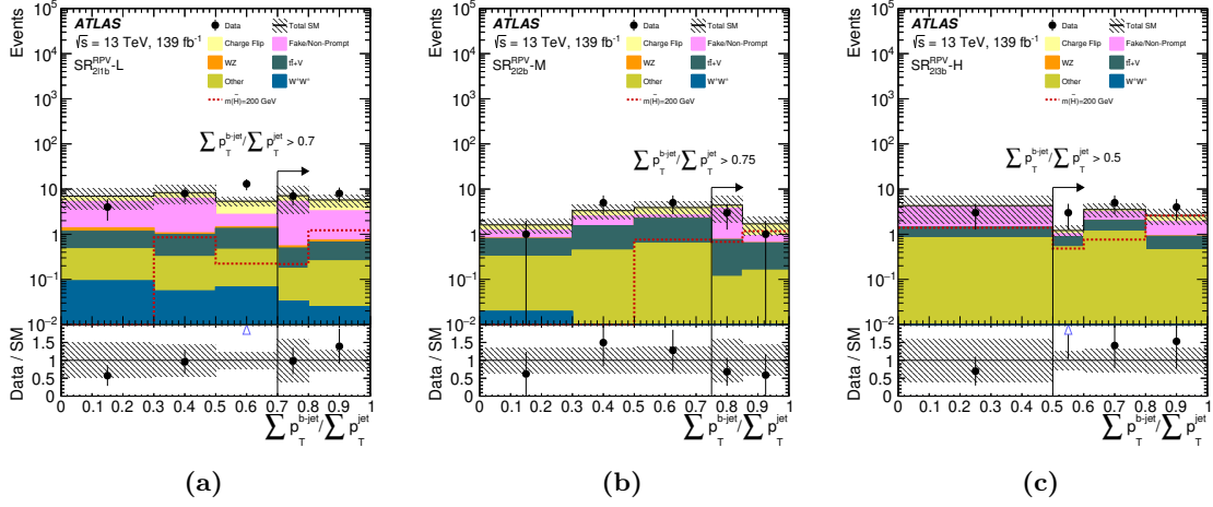
Figure 16. \Sigma p_T^{b\text{-jet}} / \Sigma p_T^{\text{jet}} distributions of the data and the expected background in some SRs defined for the UDD RPV model with data-driven methods applied. All uncertainties are considered. The vertical black lines and the corresponding arrows indicate the cuts defining those regions. The last bin includes overflow. The ‘Other’ category contains the t\bar{t}+H , rare top, triboson, and other diboson processes with the SS final state. Distributions for a representative signal mass point are overlaid. The bottom panel shows the ratio of the observed data to the predicted yields.
