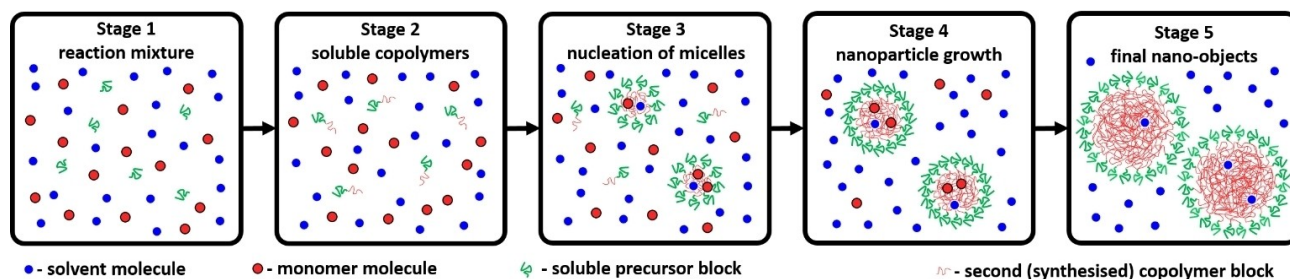
Figure 1. Schematic representation of a PISA synthesis for which the final copolymer morphology is kinetically-trapped spheres. Stage 1: Initial reaction mixture comprising solvent molecules (small blue spheres), a soluble precursor or ‘macro-CTA’ (green curves) and monomer molecules (small red spheres) that will polymerize to form the second block. Stage 2: Soluble block copolymer chains comprising a relatively short second block (red curves). [9b] Stage 3: Nucleation of micelles with the growing insoluble second block with such chains located within the micelle cores (large red spheres). Stage 4: Nanoparticle growth. Stage 5: Final spherical diblock copolymer nanoparticles.
