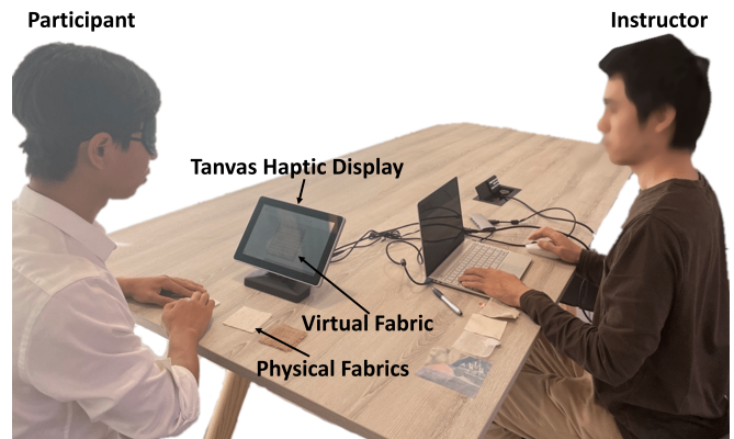
Fig. 6: Experimental setup. The participant is blinded with an eye mask and let to touch the physical fabrics on the table and the virtual fabrics on the haptic display. The instructor will change the physical and virtual fabrics and record the reaction from the participant.
