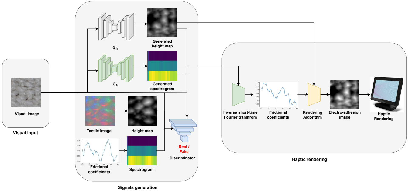
Fig. 2: Diagram of proposed haptic rendering framework. Two generators G_h and G_s are implemented to generate the height maps of object’s surface and spectrogram of frictional coefficients respectively. The discriminator is used to identify the generated tactile signals from real tactile signals. After training, the generators are capable to generate realistic tactile signals from corresponding visual images. Then, the spectrogram are transformed to the waveform using inverse short-time Fourier transform algorithm and combined with generated height map for haptic rendering.
