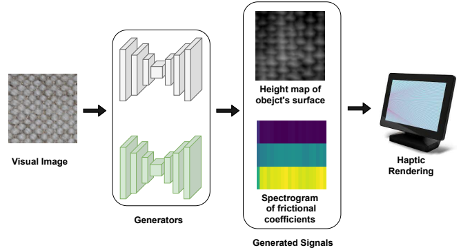
Fig. 1: Haptic rendering framework. A generative model is used to generate signals for rendering from visual images, then the generated signals are used for haptic rendering through a haptic display.
