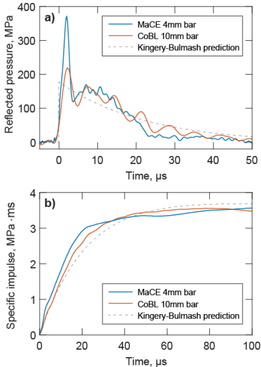
Figure 6. a) Reflected pressure and b) specific impulse measurements for a spherical PE10 charge at Z = 0.18 \text{ m/kg}^{1/3} , using 10 mm diameter pressure bars in CoBL and 4 mm diameter pressure bars in MaCE. Also shown are the semi-empirical Kingery–Bulmash predictions.
