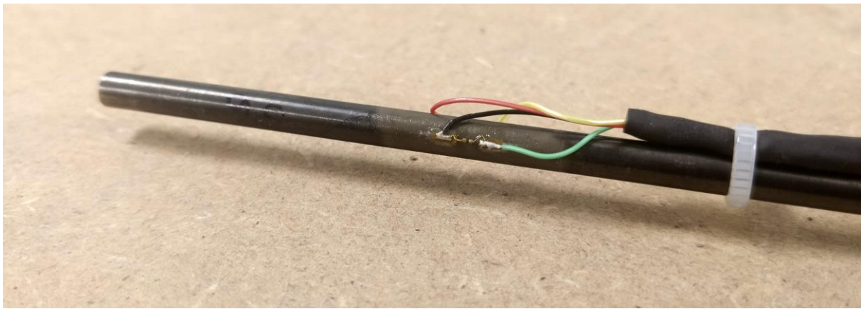
Figure 3: MaCE pressure bar. High strain capacity semiconductor gauges are bonded to a 4mm diameter maraging steel bar, 40mm from the loaded face.
