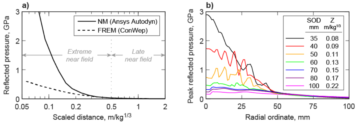
Figure 1. Predictions of near-field reflected overpressures. (a) The large discrepancy in the predictions made by numerical models such as Ansys Autodyn [10] and fast-running engineering models such as ConWep [9] in the extreme near field. (b) Numerical predictions for the peak reflected overpressure with radial ordinate on a rigid reflecting plate, resulting from a 100 g spherical charge of PE-4 at various stand-off distances.
