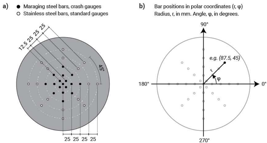
Figure 4. Central target plate pressure bar array, covering a circle with radius 100 mm. (a) Pressure bars within the inner 50 mm radius use high strength maraging 350 steel and specially manufactured “crash” gauges. Pressure bars outside the inner 50 mm radius use F51 stainless steel and standard strain gauges. (b) Polar coordinate system used to reference the bar positions, with angles measured in degrees, anticlockwise from right.
