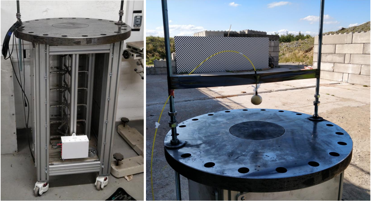
Figure 5: MaCE test frame with side panel removed, showing central pressure bar, lateral supports and electronics enclosure (left). Example of test arrangement with spherical explosive charge suspended above the target plate in glass fibre netting (right).
