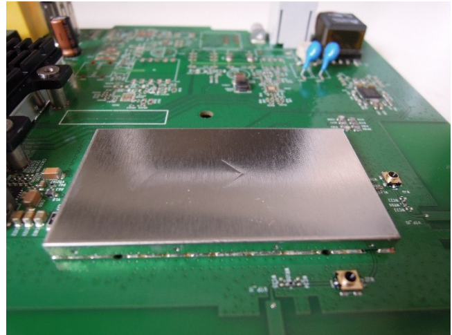
Fig. 1. Board level shield on a Wi-Fi router.
