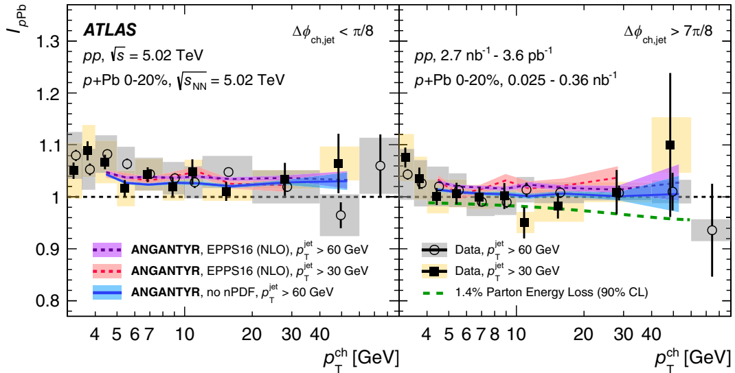
FIG. 3. The ratio of per-jet charged-particle yields, I_{p\text{Pb}} , on the near side (left) and away side (right) between p + \text{Pb} and pp are plotted for the 0%–20% p + \text{Pb} ZDC-selected centralities. Particles correlated with a jet above 30 GeV and 60 GeV are shown. Statistical uncertainties are shown as vertical lines and systematic uncertainties as filled boxes. Also shown are calculations from the ANGANTYR generator [58] with two treatments of nuclear-modified parton distribution functions (nPDFs): EPPS16 [59] at next-to-leading order and no nPDF modification, and with a PYTHIA 8-based model for parton energy loss with vacuum fragmentation (see text). ANGANTYR results are only shown for p_T^{\text{ch}} > 4.5 GeV where no UE subtraction is necessary. The colored bands represent statistical uncertainties only.
