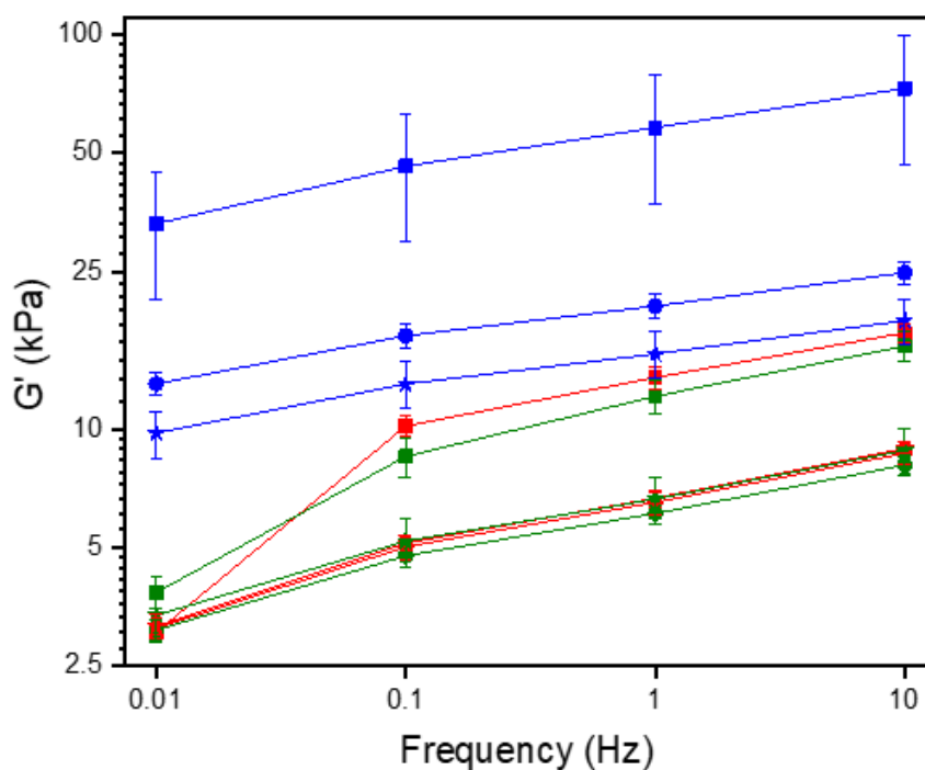
Figure 4. Mean storage modulus ( G' ) at 0.1% shear strain and 25 °C of MYC as a function of frequency showing G' with no added salts at pH 7.0 (■), 5.0 (■) and 3.0 (■); with 0.5 mM \text{Fe}_4(\text{P}_2\text{O}_7)_3 at pH 7.0 (●), 5.0 (●) and 3.0 (●); with 1.0 mM \text{Fe}_4(\text{P}_2\text{O}_7)_3 at pH 7.0 (★), 5.0 (★) and 3.0 (★). Error bars represent standard deviation for rheological analysis of triplicate samples ( n = 3 \times 3 ).
