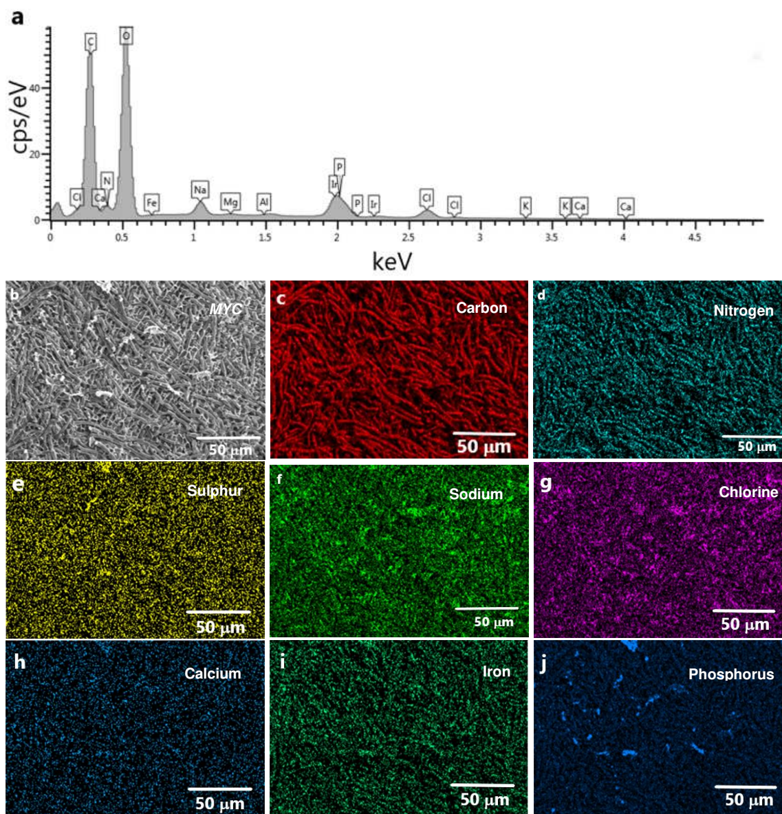
Figure 3. Elemental map of MYC (20 wt. %) with 200 mM NaCl, 100 mM CaCl 2 and 1.0 mM Fe 4 (P 2 O 7 ) 3 at pH 5.0 showing a) relative elemental composition spectra b) fungal hyphae paste c) Carbon d) Nitrogen e) Sulphur f) Sodium g) Chlorine h) Calcium i) Iron j) Phosphorus from Cryo-SEM EDX. Scale bar represents 50 µm.
