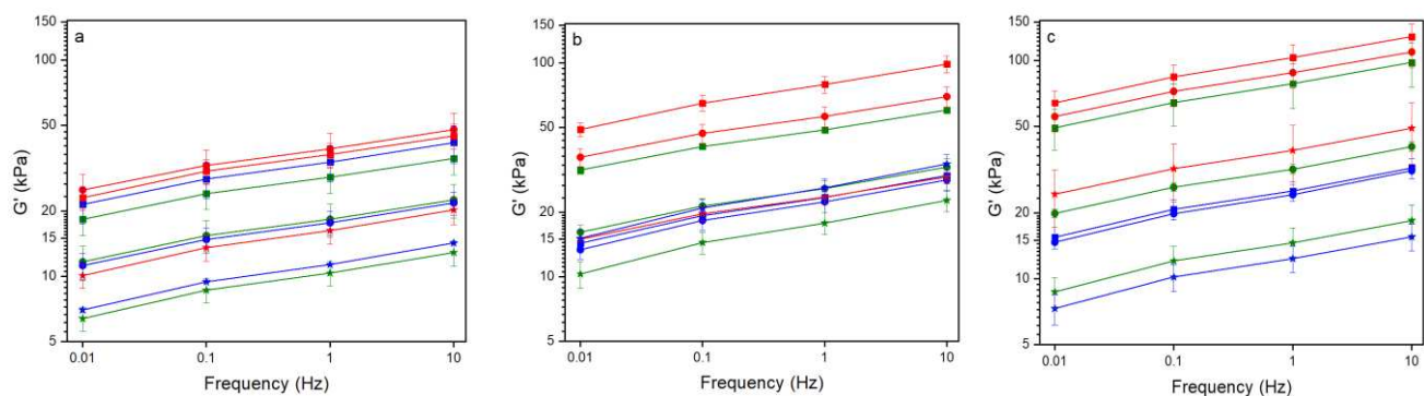
Figure S2: Mean storage modulus ( G' ) at 0.1% shear strain, 25 °C and pH 3.0 of MYC-PoP as a function of frequency showing G' with no added salts (■), 100 mM (■) and 200 mM NaCl (■); with 50 mM \text{CaCl}_2 (●), and 100 mM NaCl (●) and 200 mM NaCl (●); with 100 mM \text{CaCl}_2 (★), and 100 mM NaCl (★) and 200 mM NaCl (★); a) no added \text{Fe}_4(\text{P}_2\text{O}_7)_3 , b) 0.5 mM \text{Fe}_4(\text{P}_2\text{O}_7)_3 , c) 1.0mM \text{Fe}_4(\text{P}_2\text{O}_7)_3 . Error bars represent standard deviation for rheological analysis of triplicate samples ( n = 3 \times 3 ).
