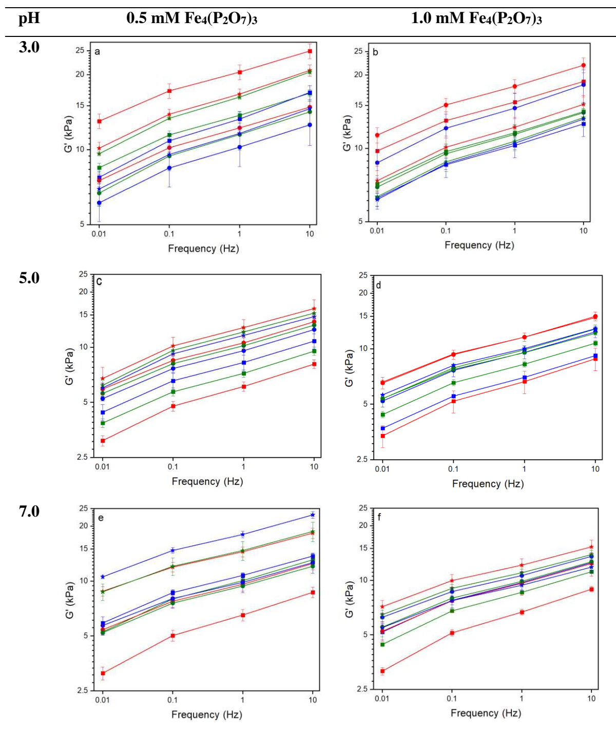
Figure S1: Mean storage modulus ( G' ) at 0.1% shear strain and 25 °C of MYC as a function of frequency showing G' with no added salts (■), 100 mM (■) and 200 mM NaCl (■); with 50 mM \text{CaCl}_2 (●), and 100 mM NaCl (●) and 200 mM NaCl (●); with 100 mM \text{CaCl}_2 (★), and 100 mM NaCl (★) and 200 mM NaCl (★) with 0.5 mM \text{Fe}_4(\text{P}_2\text{O}_7)_3 at pH a) 3.0, c) 5.0, e) 7.0; and with 1.0 mM \text{Fe}_4(\text{P}_2\text{O}_7)_3 at pH b) 3.0 d) 5.0 and c) 7.0. Error bars represent standard deviation for rheological analysis of triplicate samples ( n = 3 \times 3 ).
