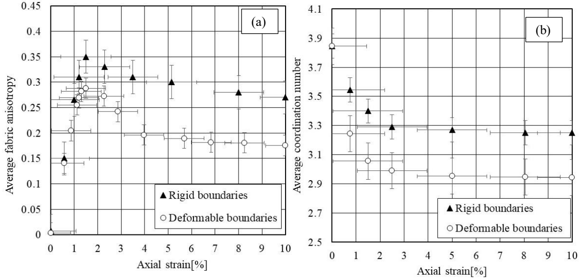
Figure 9 The sensitivity of (a) Average Fabric anisotropy and (b) average coordination number to the different boundary condition for rigid and deformable boundary
