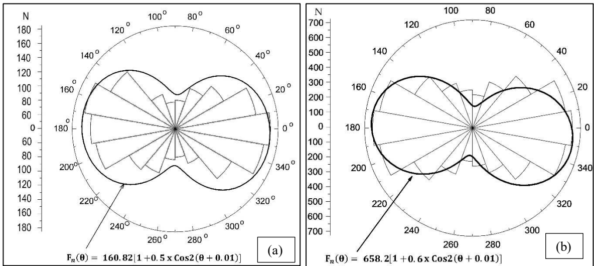
Figure 10 Normal contact force distribution at \epsilon_{11} = 10\% , (a) deformable boundary particles, (b) rigid boundary
