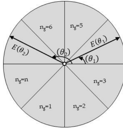
Figure 1 Schematically presentation of the concept of E(\theta) , \theta , segment, n_g highlighted in Equation 6 to Equation 8
