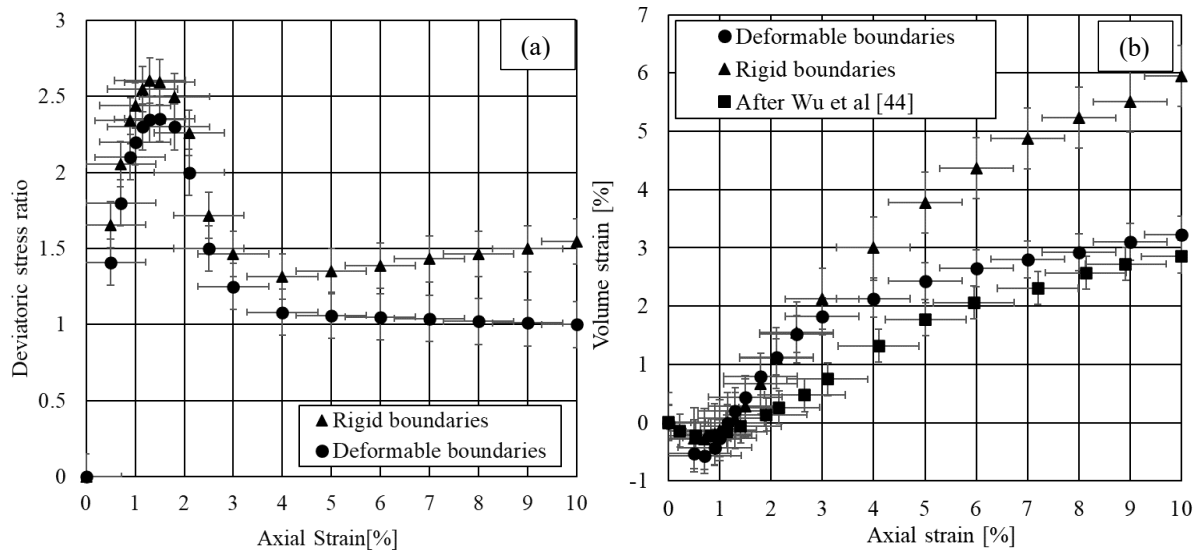
Figure 12 The sensitivity of macro-mechanical behaviour of the system to the different boundary condition: deviatoric stress ratio vs. axial strain, volumetric strain vs. axial strain
