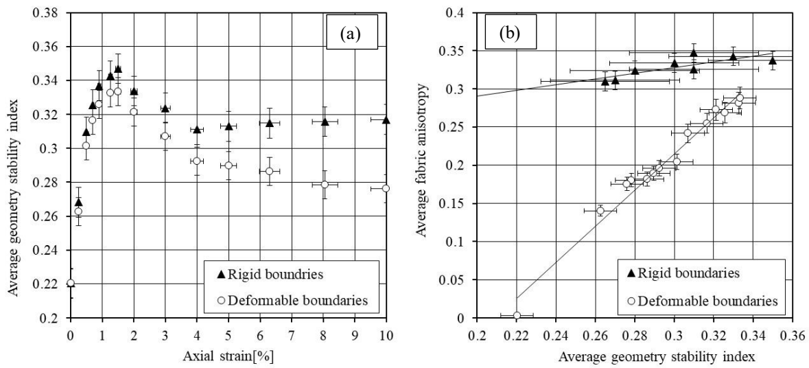
Figure 11 (a) The sensitivity of average geometrical stability index to the different boundary condition, linear coloration between average fabric anisotropy and average geometrical stability index
