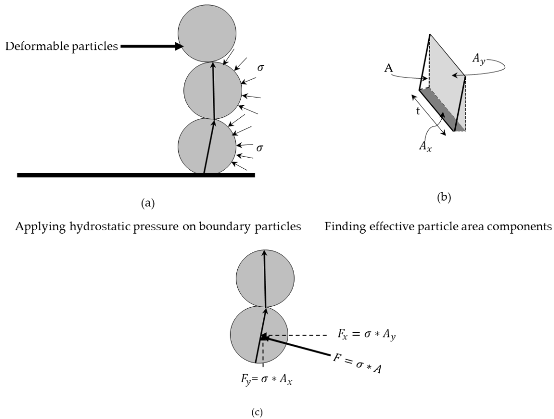
Figure 5 Applying external forces on right boundary particles schematically.
