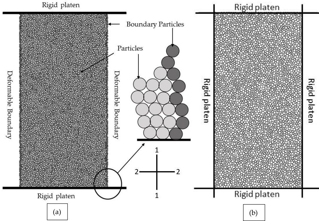
Figure 7 The biaxial sample: (a) deformable vertical boundaries, (b) rigid vertical boundaries; 1-1 and 2-2 are the direction of major and minor axis.
