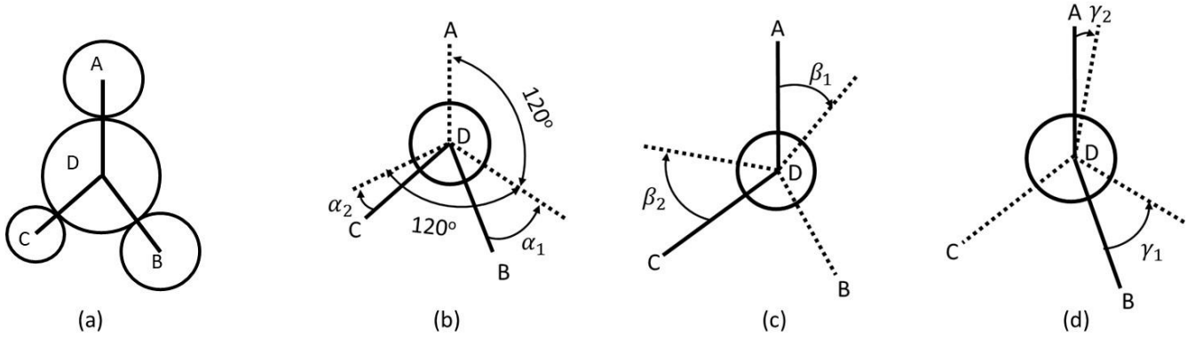
Figure 2 Concept of geometrical stability index (After Momeni et al. 2022 [1]) Therefore, there are three sets of d^{Sn} . For the first set (Figure 2b):
