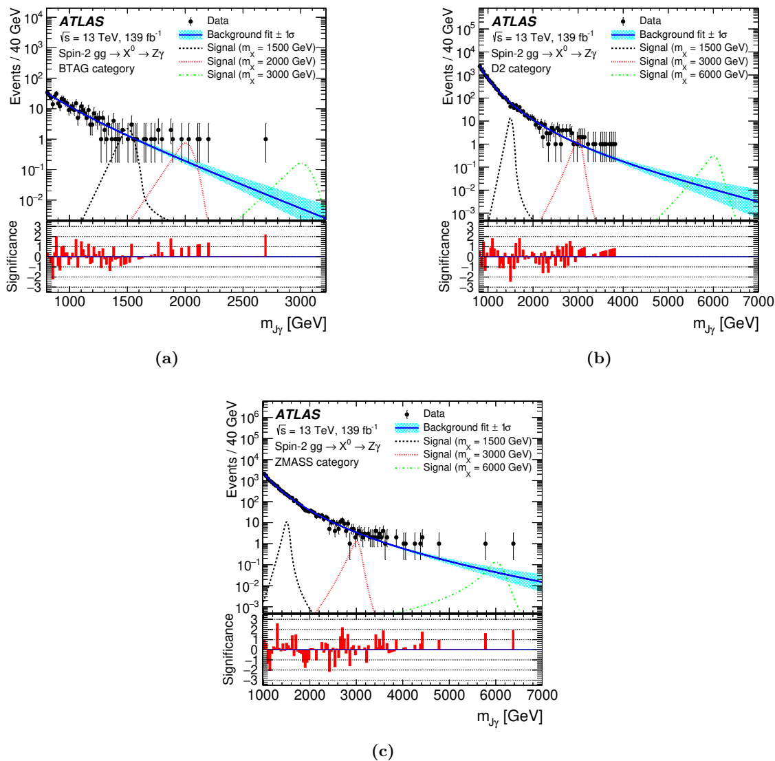
Figure 6. The m_{J\gamma} distributions of data events selected for the spin-2 gg \rightarrow X^0 \rightarrow Z\gamma search in the (a) BTAG, (b) D2, and (c) ZMASS categories. The background-only fit function shape is shown as the solid curve overlaid with a shaded band corresponding to statistical uncertainties in background parameters. Various signal shapes with cross-sections corresponding to expected limits are shown as dashed lines. The bottom panel presents the binned local significance (filled bars) from a comparison of the data with the background fit using a Poisson model [75].
