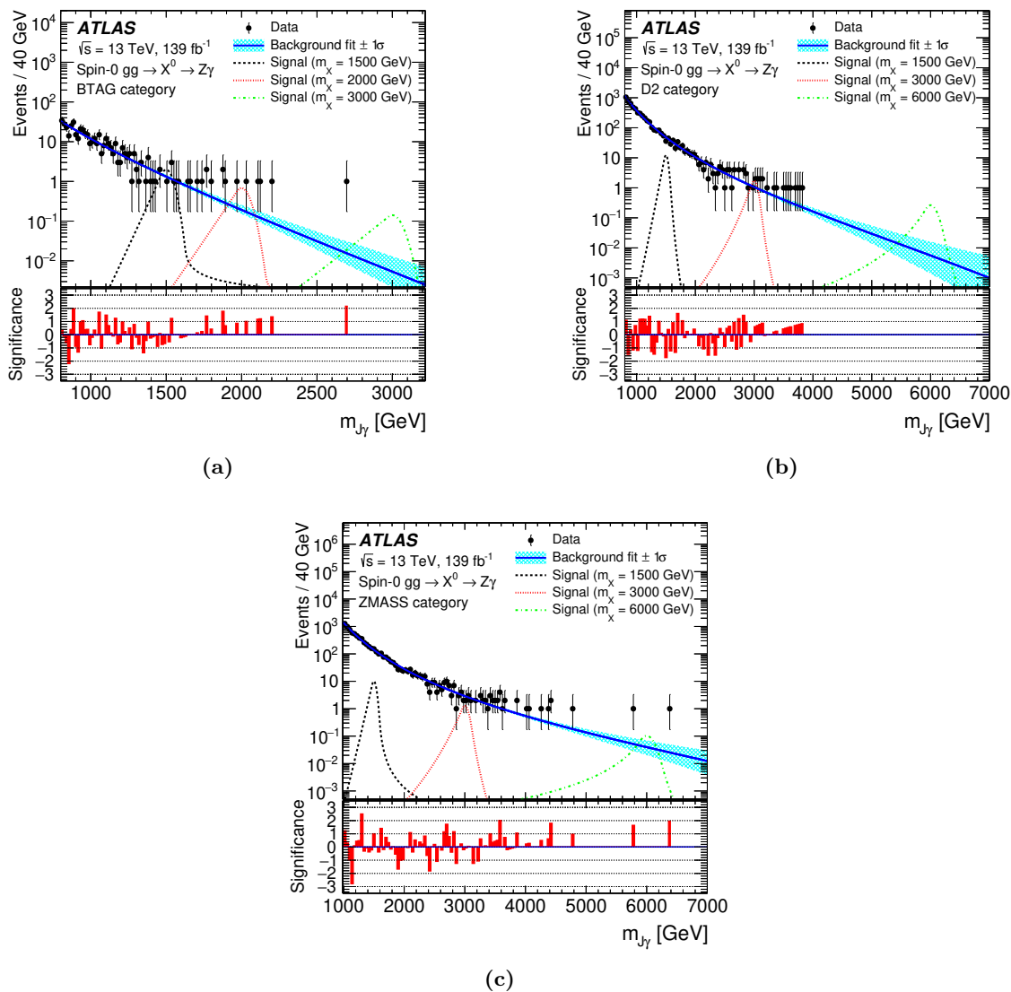
Figure 5. The m_{J\gamma} distributions of data events selected for the spin-0 gg \rightarrow X^0 \rightarrow Z\gamma search in the (a) BTAG, (b) D2, and (c) ZMASS categories. The background-only fit function shape is shown as the solid curve overlaid with a shaded band corresponding to statistical uncertainties in background parameters. Various signal shapes with cross-sections corresponding to expected limits are shown as dashed lines. The bottom panel presents the binned local significance (filled bars) from a comparison of the data with the background fit using a Poisson model [75].
