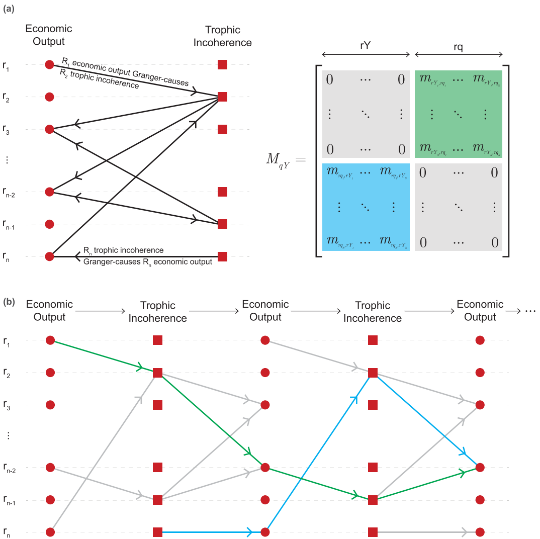
FIGURE 7 Schematic showing the assembly of a bipartite q - Y regional influence network based on Granger-causality between the two sets of variables between 2000 and 2010 (a) and an example of resulting paths of feedback reflected through the layers (b).
