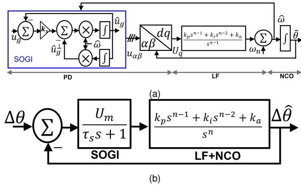
Fig. 1. Conventional single-phase SOGI-PLLs: (a) block diagram and (b) small-signal model (SSM) [11].
