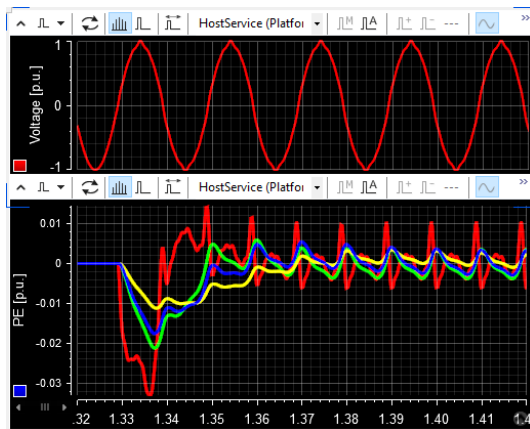
Fig. 6. Experimental results for harmonically distorted grid voltage.
