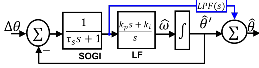
Fig. 4. Small-signal model of the proposed PLL with additional LPF.
