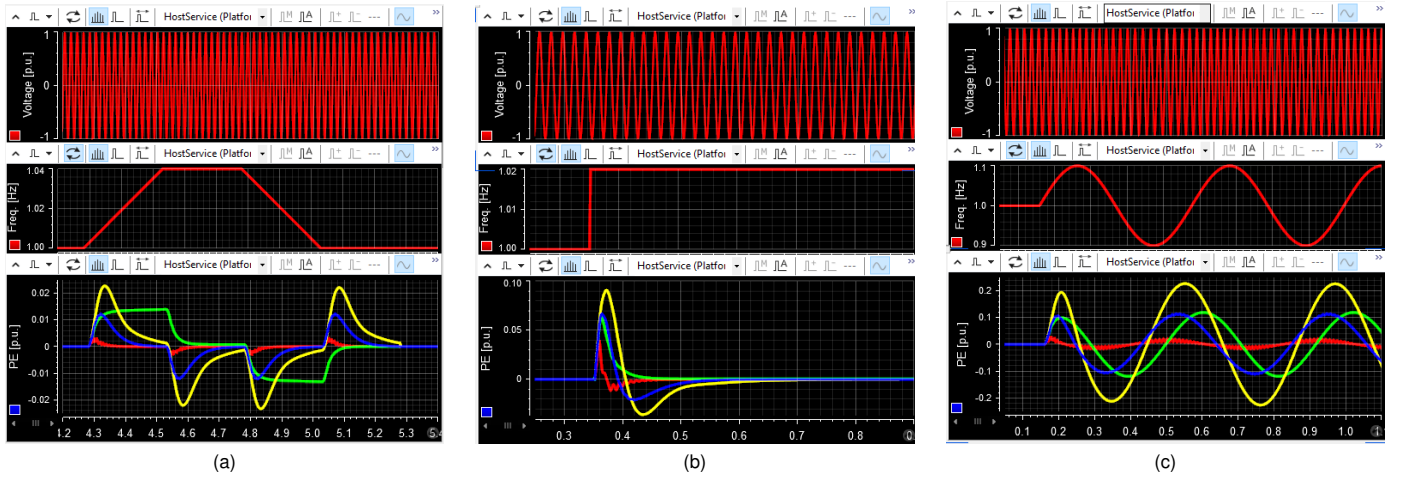
Fig. 5. Comparative experimental results for frequency variation (a) AaD, (b) step, and (c) sinusoidal.
