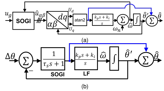
Fig. 2. Proposed QT2 SOGI-PLL: (a) block diagram and (b) SSM.
