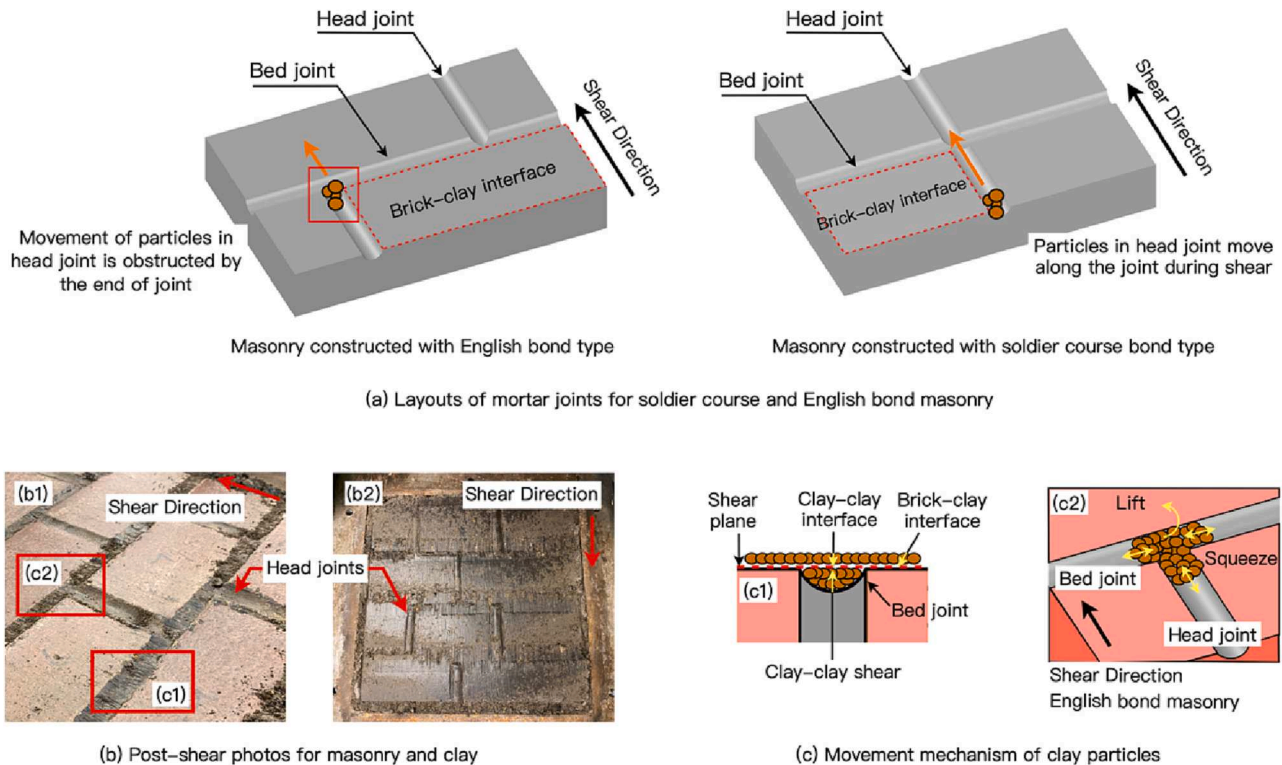
Fig. 15. (a) Layouts of mortar joints for the soldier course and English bond masonry; (b) post-shear photos for brickwork with an English bond pattern and clay; and (c) movement mechanism of clay particles during shear.
