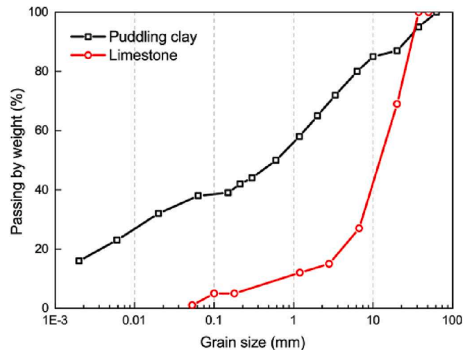
Fig. 4. Particle-size distribution of the limestone and puddling clay used in the study.
