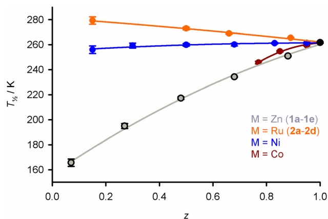
Fig. 2 Variation of T_{\frac{1}{2}} with composition in [\text{Fe}_2\text{M}_{1-z}(\text{bpp})_2][\text{BF}_4]_2 with different dopant ions, from magnetic susceptibility data measured at a 2 \text{ K min}^{-1} scan rate (Fig. 1). Data for \text{M} = \text{Ni} and \text{Co} are taken from ref. 42 and 54.
