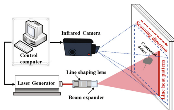
Fig. 1. Principal of Laser-line scanning thermography system.
