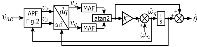
Figure 4. APF-based Quasi Type-1 PLL.
