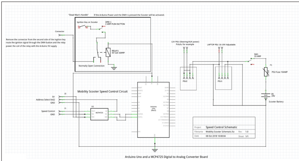
Figure 3 Circuit diagram for electronic modifications.
