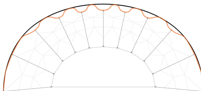
Fig.3: Outer structure members being pulled inwards with a set of wire-ropes ending to a wire mesh in tension.
