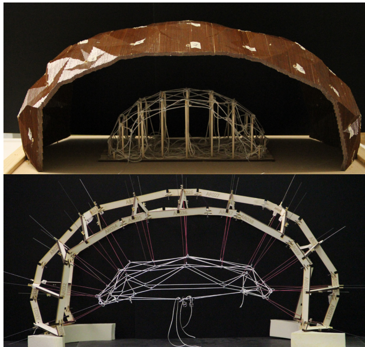
Fig. 4: Physical models were used for observing the internal wire mesh behaviour and provide input for determining the resulting geometry.
