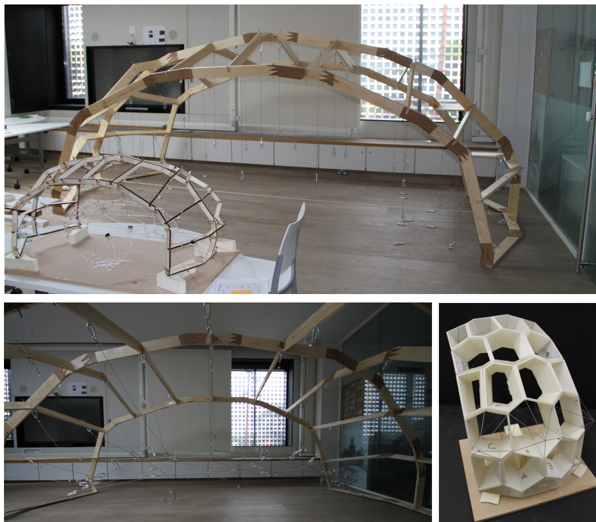
Fig.11: Structure and prototypes.
