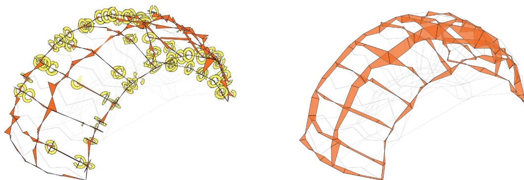
Fig.9: Resulting final diagrams of bending moments and torsion (left) and of deflections (right) following the geometric methods applied.
