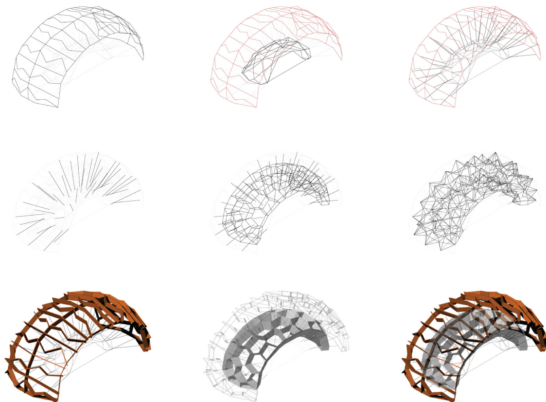
Fig.2: Diagrams showing member categories and assembling sequence (top row). Outer skeleton (birch plywood) connects with the internal wire mesh with additional wire ropes each one carrying a voronoi-cell waterproof fabric element. Bounding box dimensions: 5m, 2.5m, 2.2m (height).
