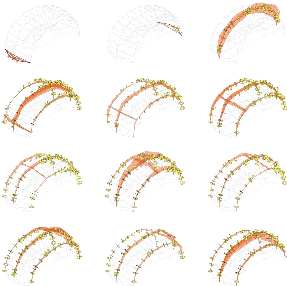
Fig.8: Display of the geometric loop-based method for distributing force and for visualising bending moments and torsion. The superimposition of the diagrams provides the total bending and torsion applied.
