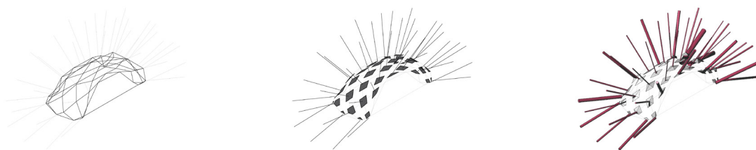
Fig.7: Introducing the Doo-Sabin mesh subdivision for determining force, the areas of the polygonal geometries created are assumed to provide the amount of force for each wire in tension; pipe diameters graphically show the deviation from OasysGSA values.
