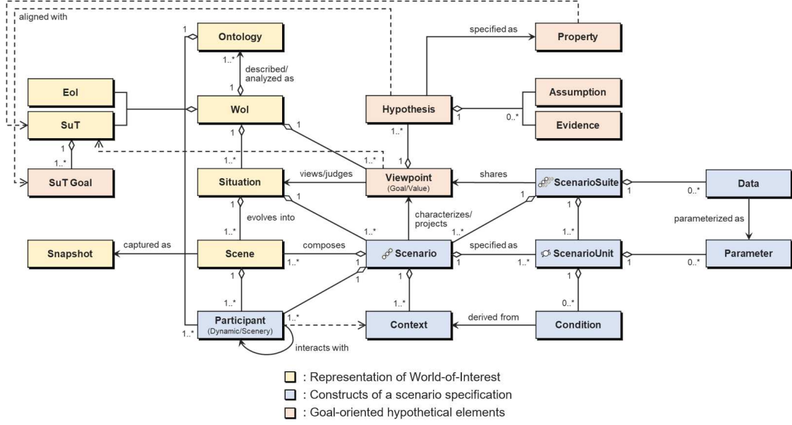
Figure 8: A CSM and three aspects of scenario methods
