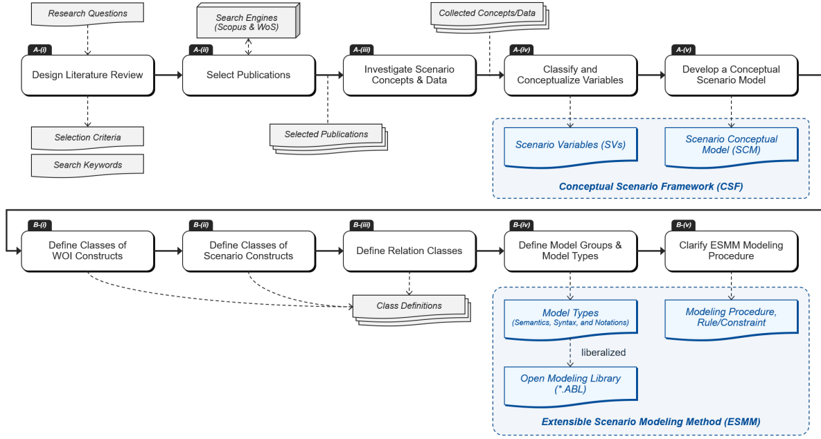
Figure 5: Overall Approach
