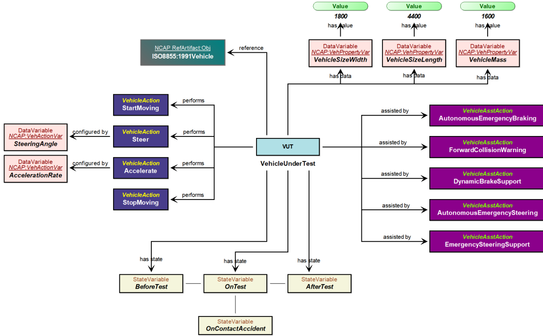
Figure 20: A type definition model (VUT) developed using SML-ER-NCAP
