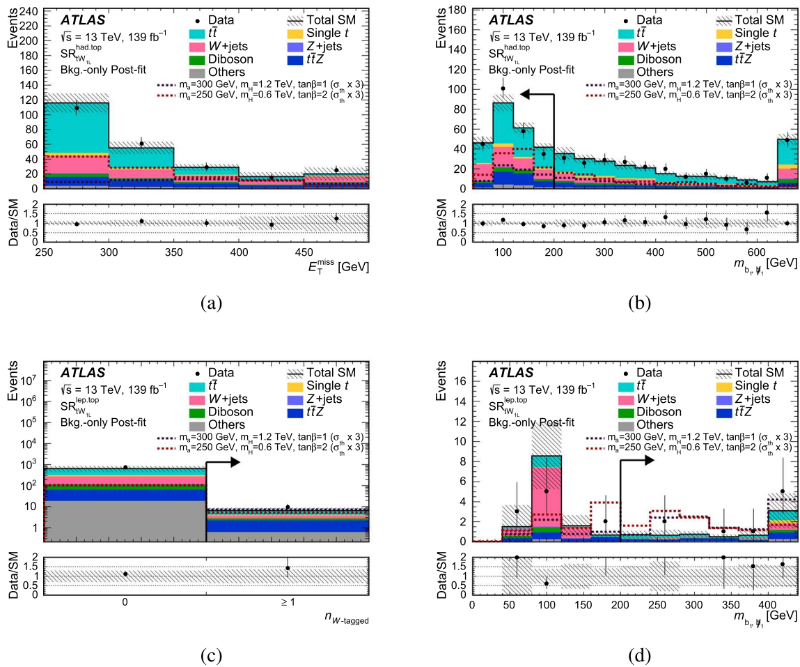
Fig. 9 Representative distributions of a E_T^{\text{miss}} and b m_{b_1, \psi_1} in \text{SR}_{tW_{\text{IL}}}^{\text{had, top}} , as well as c the number of W -tagged large- R jets and d m_{b_1, \psi_1} in \text{SR}_{tW_{\text{IL}}}^{\text{lep, top}} . Observed data are compared with the SM background predictions extrapolated from the background-only fit. The ‘Others’ category includes contributions from rare processes such as tWZ , tZ , triboson, t\bar{t}t , t\bar{t}\bar{t} , t\bar{t}W and t\bar{t}H . The expected distributions for representative scenarios with different m_a , m_{H^\pm} , and \tan\beta values are shown for illus-
