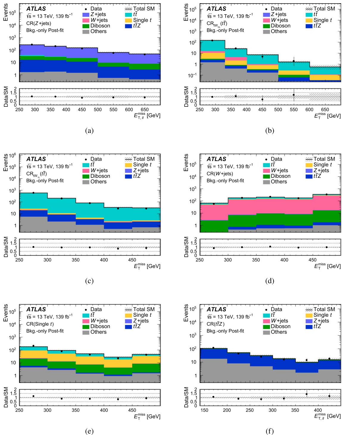
Fig. 3 The post-fit E_{T,miss} and E_{T,miss, ll} distributions in the a Z+jets, b tW_{0L} t\bar{t} , c tW_{1L} t\bar{t} , d W+jets, e single-top, and f t\bar{t}Z control regions. The last bin in the histogram includes the overflow events. The bottom panel shows the ratio of data to total SM background. The uncertainties
