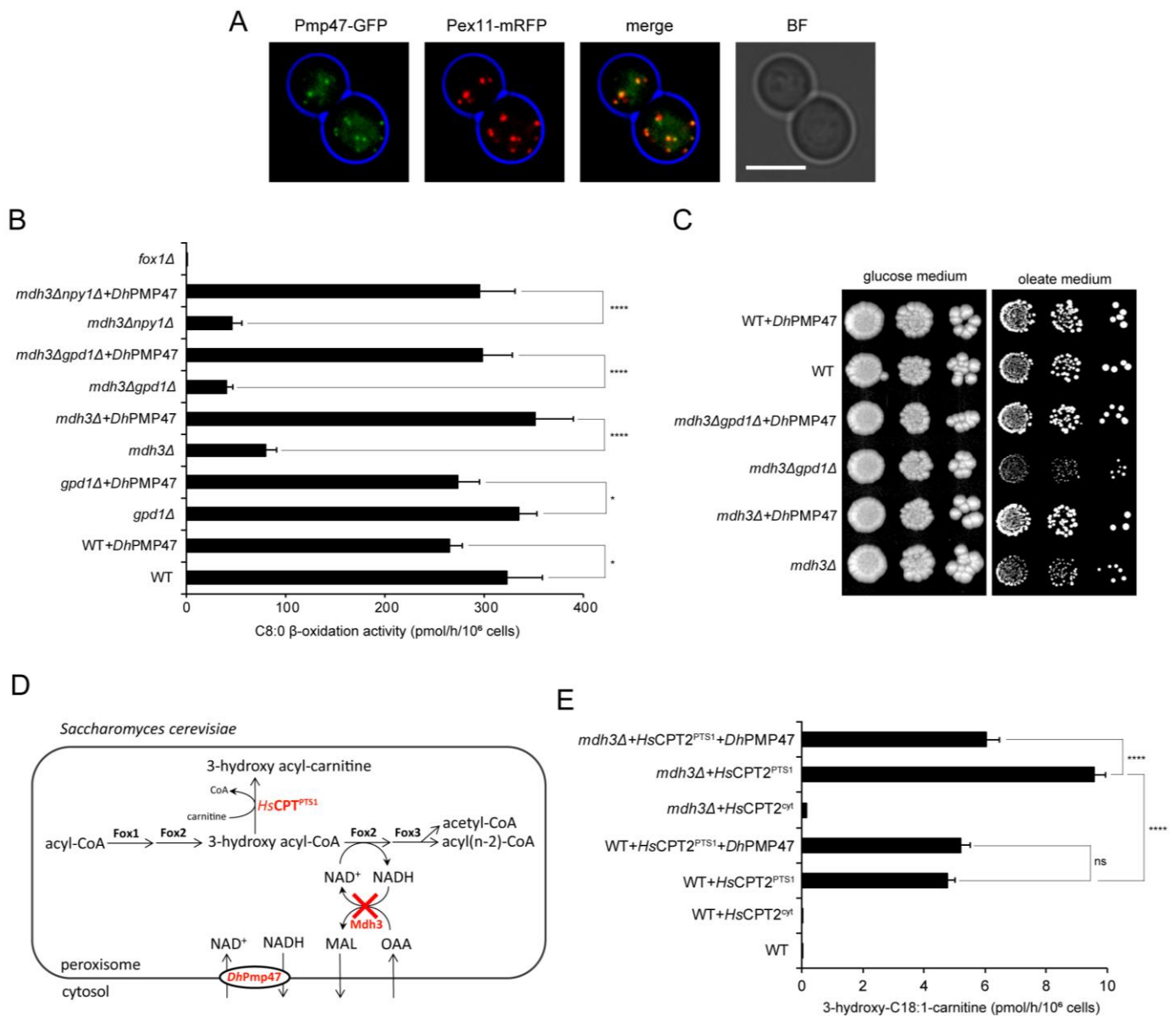
Figure 4. DhPmp47 is a peroxisomal NAD + carrier involved in the maintenance of peroxisomal NAD + required for β-oxidation. (A) DhPmp47-GFP was localised to the peroxisomal membrane upon expression in S. cerevisiae cells. Representative epifluorescence microscopy images of wild-type S. cerevisiae cells expressing the peroxisomal membrane marker, Pex11-mRFP, and DhPmp47 fused with GFP (DhPmp47-GFP). Red and green channel images are merged z-stacks. Merge is an overlay of the red and green merged z-stacks. Bright-field (BF) images were collected in one plane and were processed to highlight the cell circumference in blue in other panels. Scale bar: 5 μm. (B,C,E) DhPmp47 was expressed in wild-type or mutant S. cerevisiae cells behind an oleate-inducible CTA1 promoter. (B) Heterologous expression of DhPmp47 rescued the β-oxidation activity of mdh3Δ , mdh3Δgpd1Δ and mdh3Δnpy1Δ S. cerevisiae cells. S. cerevisiae cells were oleate-induced (grown overnight on oleate medium), and β-oxidation rates were measured using [1- 14 C]-labelled octanoate as substrate. The results are shown as mean ± standard deviation (n = 4). One-way ANOVA with Tukey’s multiple comparisons test was performed to determine if differences were significant. Cells transformed with empty plasmid and fox1Δ cells, deficient of the first enzyme of the β-oxidation pathway, were used as controls. (C) Heterologous expression of DhPmp47 rescued the ability of mdh3Δ and mdh3Δgpd1Δ S. cerevisiae cells to utilise oleate. Growth analysis of the indicated S. cerevisiae strains either expressing DhPmp47 or transformed with an empty plasmid on media containing glucose or oleate as sole carbon source. (D) Schematic representation of the peroxisomal
