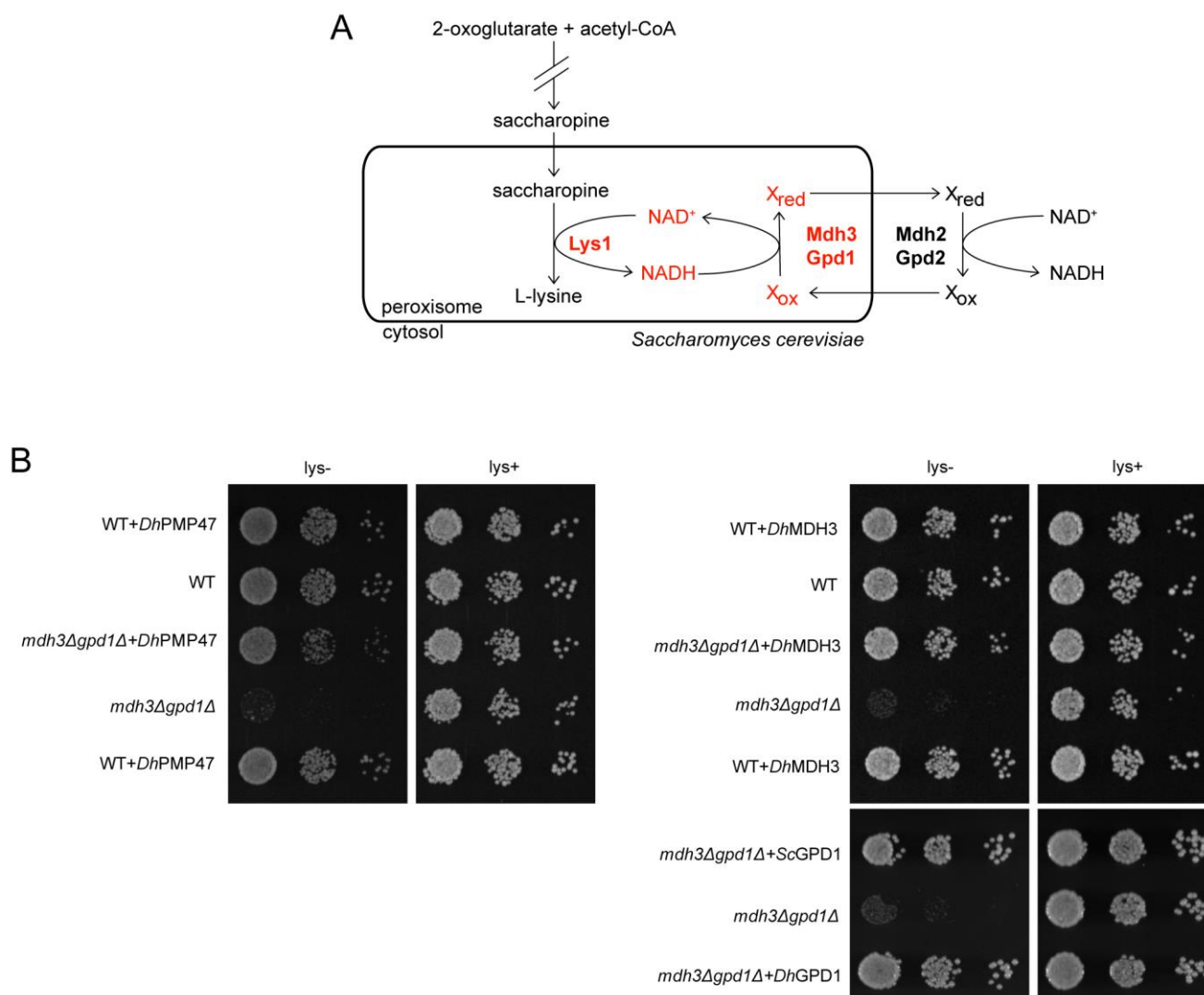
Figure 5. Heterologous expression of DhPmp47 supplies S. cerevisiae peroxisomes with \text{NAD}^+ required for lysine biosynthesis. (A) Schematic representation of the peroxisomal step of lysine biosynthesis pathway in S. cerevisiae . A deletion of Mdh3 and Gpd1 enzymes, that are part of the peroxisomal malate and glycerol-3-phosphate redox shuttles, results in a deficiency in lysine biosynthesis. (B) Lysine bradytrophism (slow-growth phenotype on lysine-free medium) was repressed by heterologous expression of DhPmp47 , DhMdh3 and DhGpd1 in S. cerevisiae mdh3Δgpd1Δ cells. Growth analysis on glucose medium in the absence or presence of lysine. Wild-type and mdh3Δgpd1Δ cells were transformed with plasmids encoding DhPmp47 , DhMdh3 , DhGpd1 -GFP, ScGpd1 -GFP or empty plasmid.
