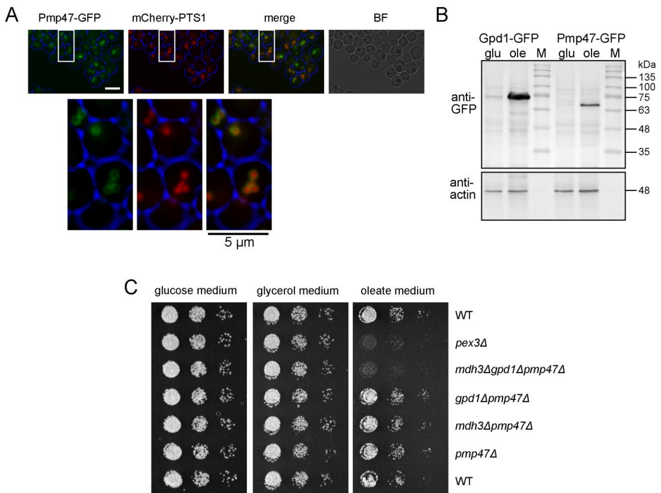
Figure 3. Pmp47 is a peroxisomal protein that contributes to fatty acid \beta -oxidation in D. hansenii . (A) Representative epifluorescence microscopy images of wild-type D. hansenii cells expressing mCherry-PTS1 and Pmp47-GFP expressed from its chromosomal locus. Cells were grown on oleate medium for 6 h. Red and green channel images are merged z-stacks. Merge is an overlay of the red and green merged z-stacks. Bright-field (BF) images were collected in one plane and are processed to highlight the cell circumference in blue in other panels. The white rectangles are enlarged below to show the ring-like GFP signal of Pmp47-GFP, which surrounds the peroxisomal lumen stained with mCherry-PTS1. Scale bar: 5 \mu m. (B) Western blot analysis of lysates of wild-type D. hansenii cells expressing Gpd1-GFP or Pmp47-GFP under control of their endogenous promoter grown on glucose (glu) or oleate (ole) media using anti-GFP and anti-actin (loading control). Protein ladder (M) was used as size standard. (C) Growth analysis of wild-type and mutant D. hansenii cells on media containing glucose, glycerol or oleate as sole carbon sources.
