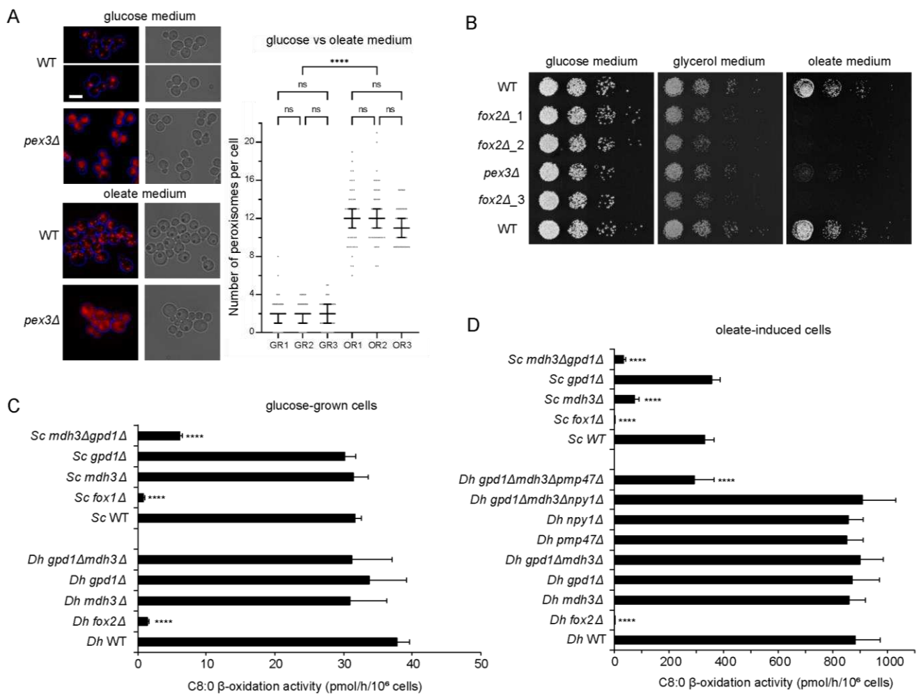
Figure 1. D. hansenii peroxisomes are required for the utilisation of fatty acids as a carbon source via \beta -oxidation. (A) Peroxisome number increased when D. hansenii cells were grown on oleate-based medium. Representative epifluorescence microscopy images of wild-type and pex3Δ cells expressing mCherry-PTS1 and grown on glucose medium to exponential growth phase or grown on oleate medium for 6 h. Red channel images are merged z-stacks. Peroxisome numbers were quantified for >50 budding wild-type cells per replica (n = 3, individual replicas are labelled as GR (glucose medium replica) and OR (oleate medium replica)). Bars in the graph indicate the median with 95% confidence intervals for mean. Statistical significance analysis was performed using Kruskal–Wallis test. Scale bar: 5 \mu m. (B) Growth analysis of wild type, fox2Δ (three independent strains) and pex3Δ D. hansenii cells, on media containing glucose, glycerol or oleate as sole carbon sources. (C,D) \beta -oxidation activity was higher in oleate-induced cells compared to glucose-grown cells, and loss of Fox2 affected \beta -oxidation activity in D. hansenii cells. NAD + availability in D. hansenii was not solely dependent upon the Mdh3 and Gpd1 redox shuttles but also on Pmp47. The presented data relate to Sections 3.1–3.3 of this manuscript. \beta -oxidation activity in wild-type and mutant S. cerevisiae and D. hansenii cells, grown on (C) glucose-based medium or (D) oleate-based medium (oleate-induced cells), were measured using [1- 14 C]-labelled octanoate (C8:0) as substrate. The results are shown as mean \pm standard deviation (n = 4). One-way ANOVA with Dunnett’s multiple comparisons test was performed to determine if differences were significant when compared with the corresponding wild-type cells. ns, not significant; **** p < 0.0001.
