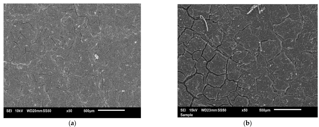
Figure 9. SEM images showing the surface morphology of Toray TGP-H-60 coated with (a) Vulcan XC-72R and (b) Ketjenblack EC-300J for MPL ink homogenisation time of three hours [29].
