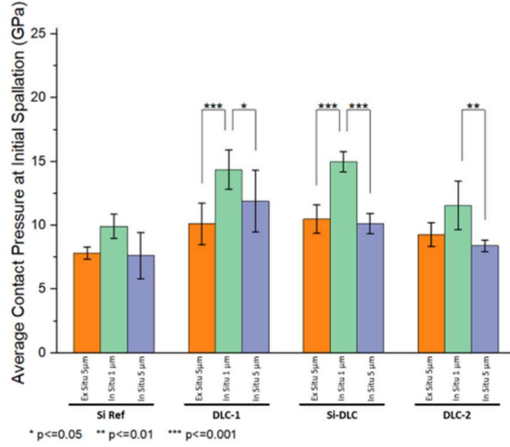
Fig. 13. Average normal contact pressure measured at the spallation onset of DLC-1, Si-DLC, DLC-2 coatings and Si reference sample, across all 5 \mu\text{m} and 1 \mu\text{m} diamond tip scratch tests. Asterisks indicate a statistical difference * p < 0.05 , ** p < 0.01 , *** p < 0.001 , obtained using Tukey test, which computes a confidence interval for the difference between two means.
