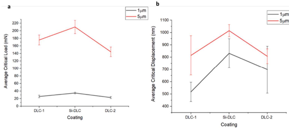
Fig. 14. Average critical normal loads and corresponding diamond tip displacements measured for the onset of spallation of DLC-1, Si-DLC, DLC-2 coatings, dependent on diamond tip radius (1 \mu\text{m} and 5 \mu\text{m} ). (a) Average critical load of spallation. (b) Average critical tip displacement at spallation.
