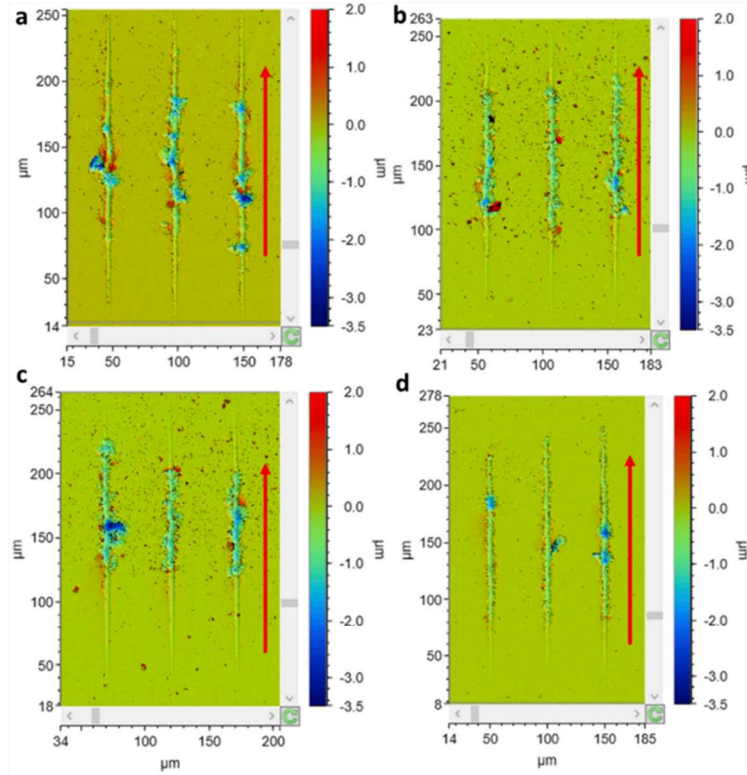
Fig. 3. Post-mortem 3D optical profilometry scans of the ex situ 5 µm diamond scratch tests. (a) Si-reference, (b) DLC-1, (c) Si-DLC, (d) DLC-2. Red arrows represent scratch direction directions and the colour bar the relative vertical (z) height. The left-hand scratch on each coating corresponds to Fig. 2. (For interpretation of the references to colour in this figure legend, the reader is referred to the Web version of this article.)
