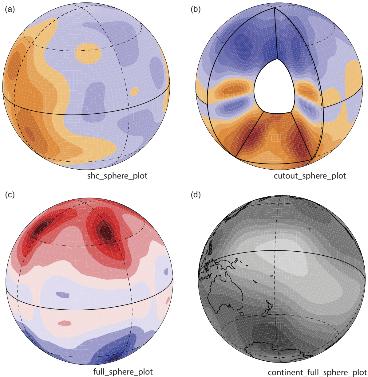
Figure 5. Example outputs from the spherical surface plotting programs listed in Section 4.3 The plots in panels (a), (b), (c), and (d) can be generated using the solution vectors and input files in the directories of the distribution GRAPHICS_shc_sphere_plot, GRAPHICS_cutout_sphere_plot, GRAPHICS_full_sphere_plot, and GRAPHICS_continent_full_sphere_plot, respectively. All documentation for each program is contained within a pdf file in the appropriate directory.
