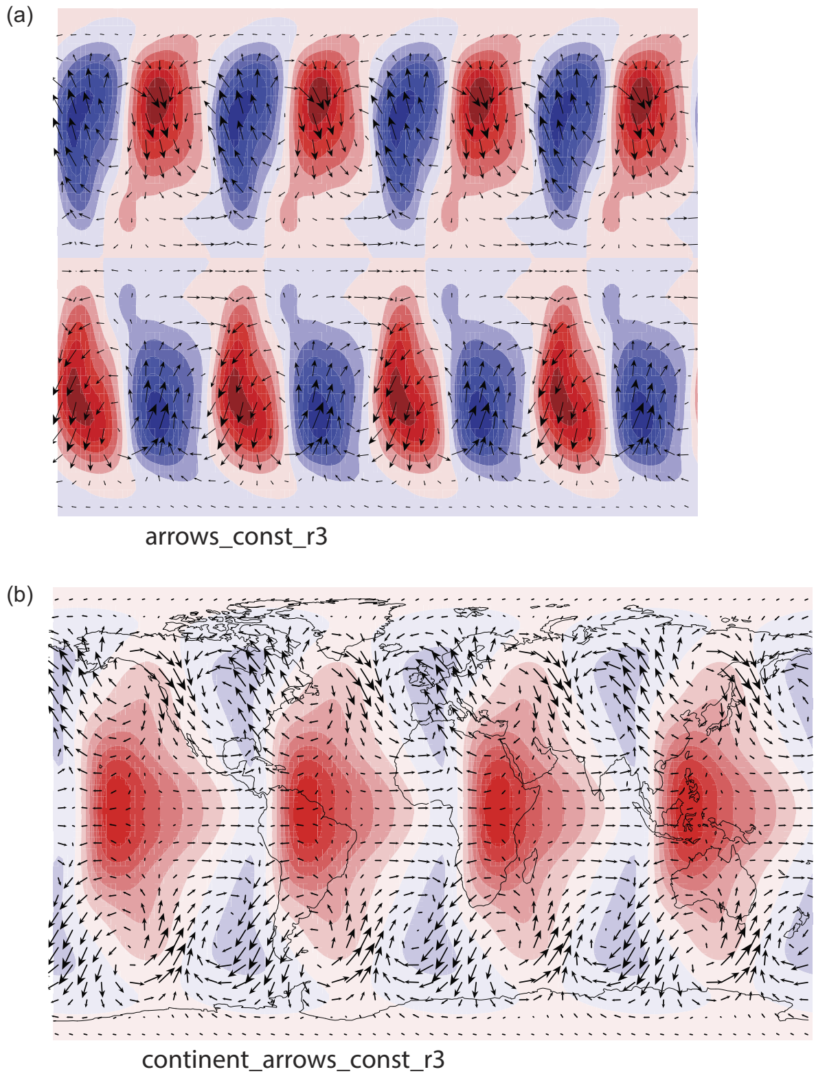
Figure 3. Example outputs from the constant radius plotting programs listed in Section 4.1 Panel (a) shows arrows of flow and coloured contours of v_\theta for the Case 0 Dynamo Benchmark study of Christensen et al. (2001) generated using the solution vector and an input file in the directory GRAPHICS_arrows_const_r3 of the distribution. Panel (b) shows contours of the temperature perturbation together with outlines of continents and arrows of flow for the same solution from the directory GRAPHICS_continent_arrows_const_r3 of the distribution. All documentation for each program is contained within a pdf file in the appropriate directory.
