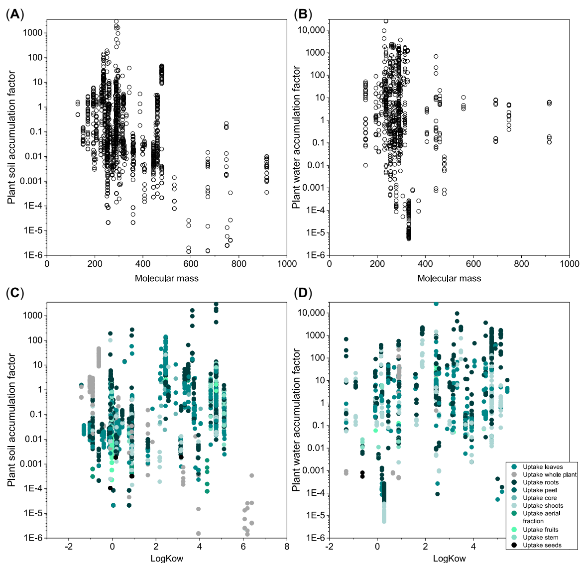
FIGURE 5: Association between plant soil accumulation factor or plant water accumulation factor and respective molecular mass ( A and B ) or log octanol–water partition coefficient (log K_{OW} ; C and D ) of pharmaceutical compounds investigated in uptake studies into crops.
