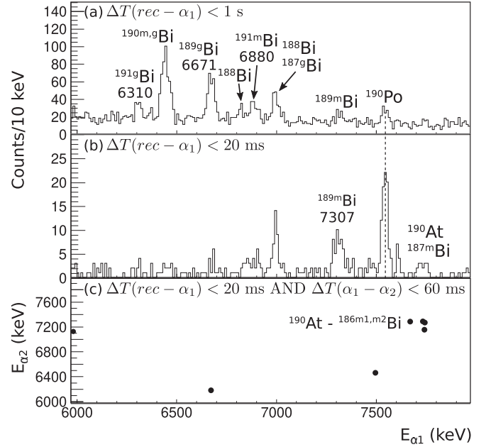
FIG. 2. Energy spectra of first generation \alpha_1 -decay events following recoil implantation within (a) 1 s and (b) 20 ms, respectively. The peaks are labeled with their energies (in keV) and the nuclide they originate from. (c) Correlation between the energies of first and second generation \alpha decays, \Delta t(\alpha_1 - \alpha_2) \leq 60 \text{ ms} .
