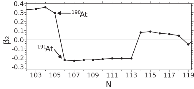
FIG. 1. Theoretical quadrupole ground-state deformation \beta_2 values for ^{188-204}\text{At} isotopes based on the macroscopic-microscopic model [8].
