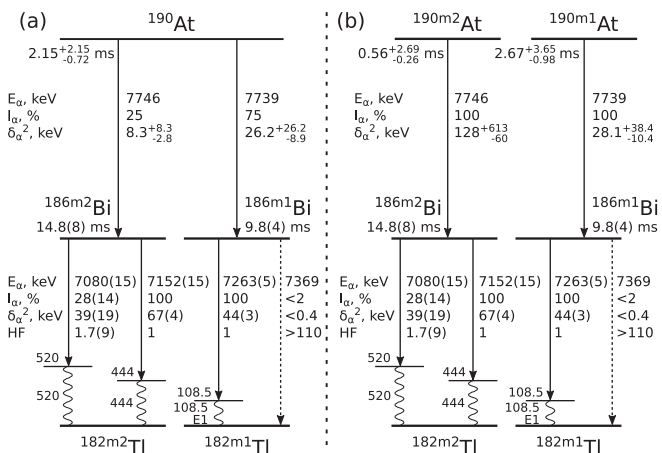
FIG. 3. Two proposed scenarios for the ^{190}\text{At} level scheme. See text for details. Decay schemes for the states in the daughter ^{186}\text{Bi} isotope were taken from Ref. [7].
