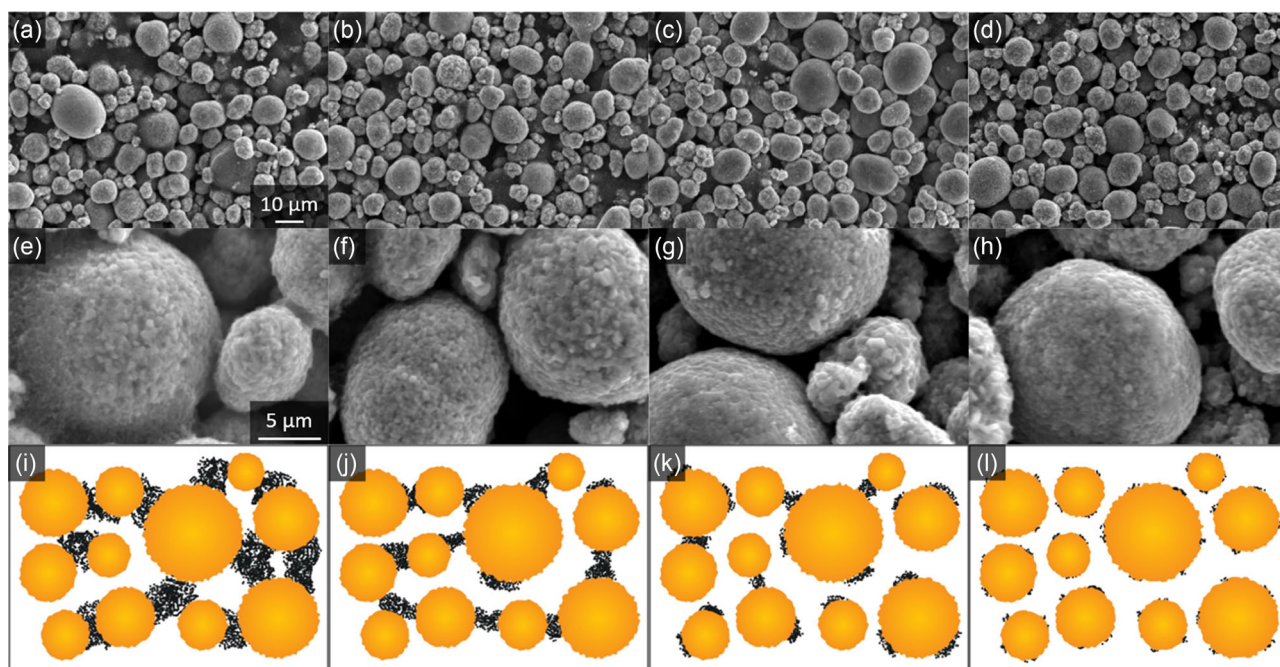
Figure 3. SEM images and schematic diagram of electrodes prepared from formulations (NMC622: carbon black: PVDF) a,e,i): 94:4:2; b,f,j): 95:3:2; c,g,k): 96:2:2; d,h,l): 97:1:2.
