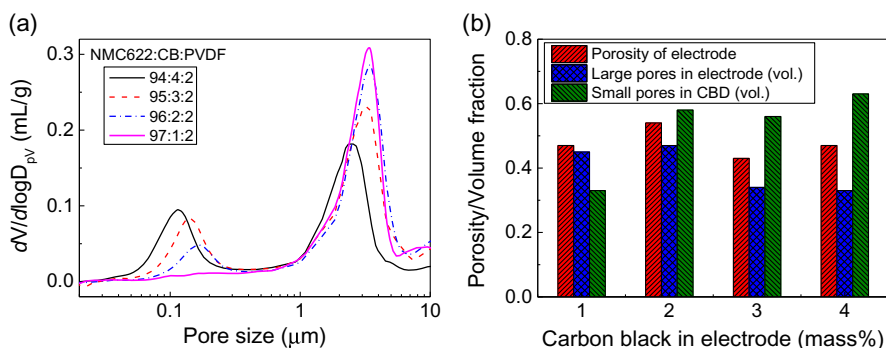
Figure 7. a) Pore size distribution measured using MIP showing changes in CBD pore size as additive content increases. b) Data extracted show overall porosity, CBD small pore, and electrode large pore volume fraction.
