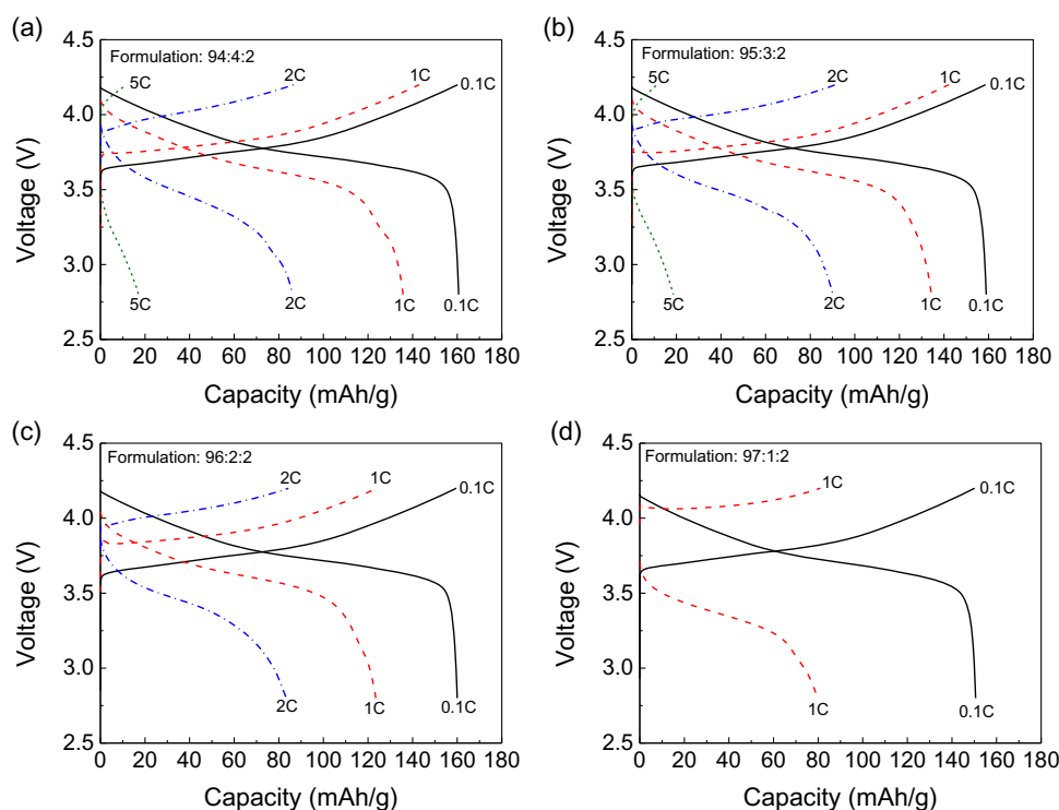
Figure 9. Charge–discharge curves for the calendared cathodes based on different electrode formulations. a–d) 94–97 wt% active material, respectively.
