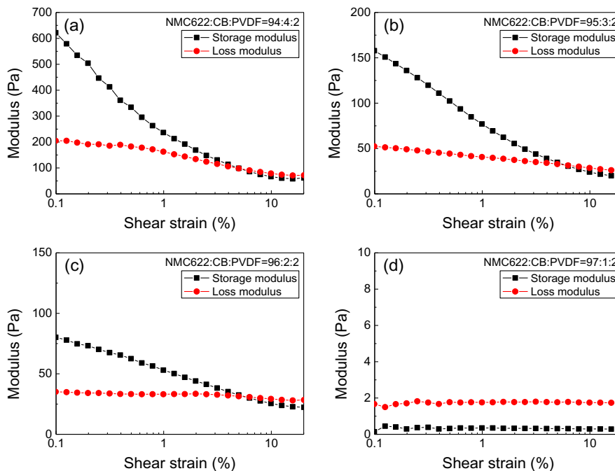
Figure 2. Storage modulus and loss modulus under strain sweeping and frequency sweeping for different formulations. a–d) 94–97 wt% active material, respectively.
