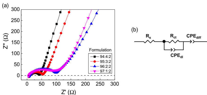
Figure 8. EIS of the electrodes a) impedance; b) equivalent circuit.
