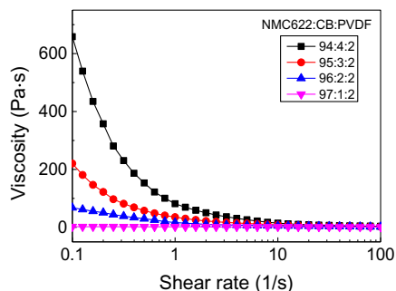
Figure 1. Relationship between viscosity and shear rate for different formulations.
