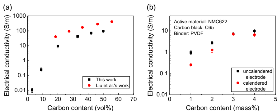
Figure 6. Electrical conductivity of carbon black in PVDF and electrodes a) composites of carbon black and PVDF in comparison with ref. [44]; b) NMC622 electrodes.
