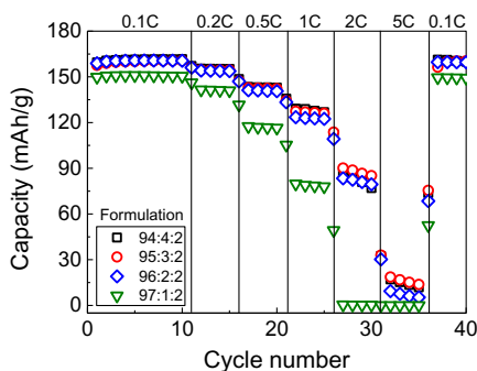
Figure 10. Rate capabilities for the calendared cathodes based on different electrode formulations.
