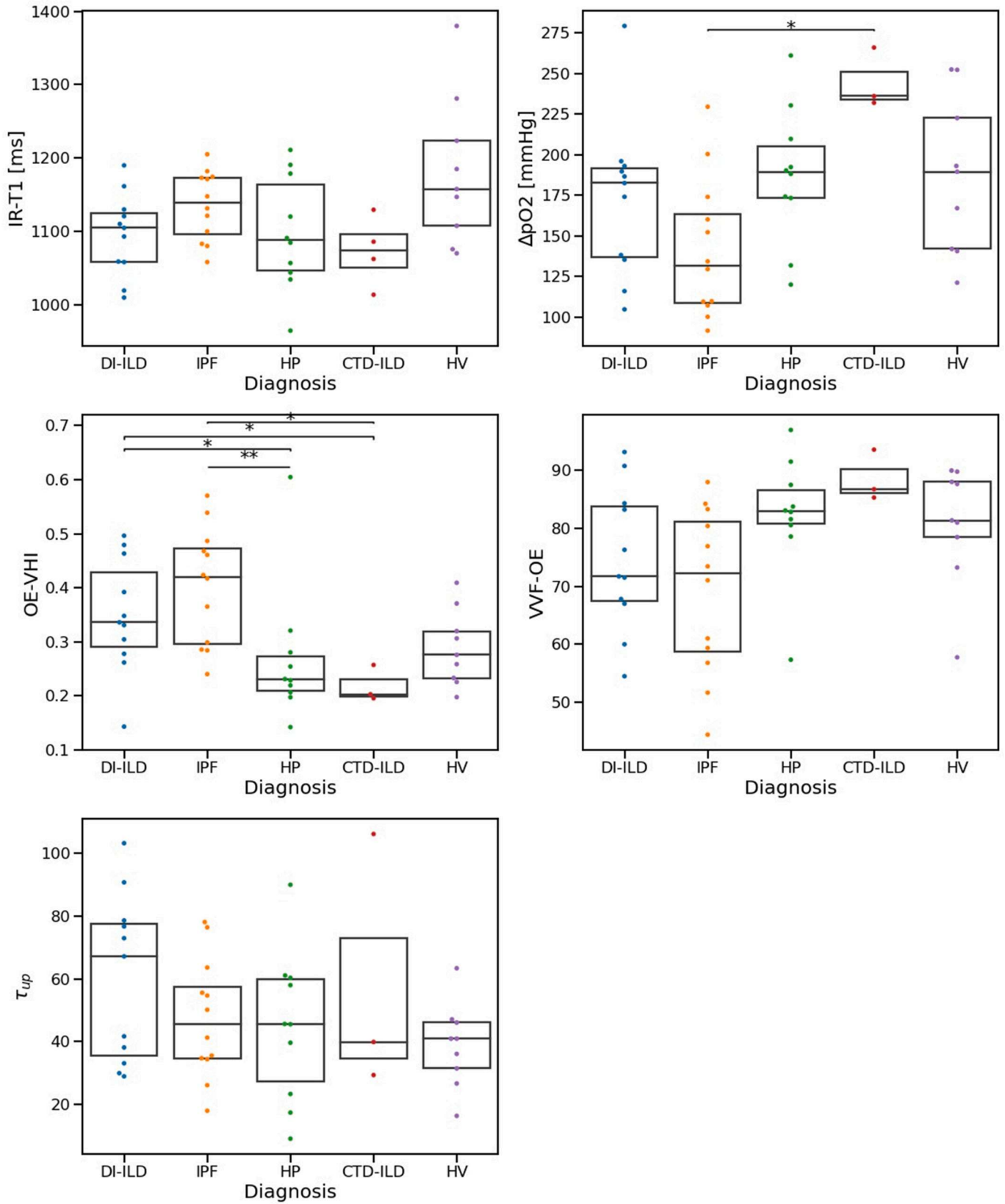
Fig. 7. Boxplot of pulmonary proton MR biomarkers at visit 1 in the studied population, split in ILD subgroups. (*) p < 0.05 , (**) p < 0.01 . \Delta pO_2 : change in oxygen partial pressure, \tau_{up} : wash-in rate of oxygen, OE-VVF: percentage of ventilated volume as calculated by oxygen-enhanced MRI, OE-VHI: ventilation heterogeneity index as calculated by oxygen-enhanced MRI, T_1 : inversion recovery T_1 .
