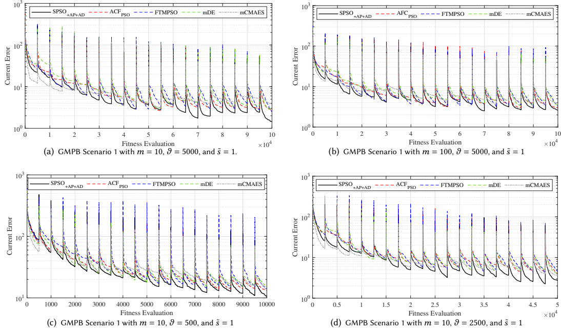
Fig. 1. Current error plots of SPSO+AP+AD, ACF PSO , FTMPSO, mDE, and mCMAES on four problem instances generated by GMPB Scenario 1 with different configurations and for 20 environments. All sub-figures are illustrated according to the average of the current errors for 31 independent runs.
