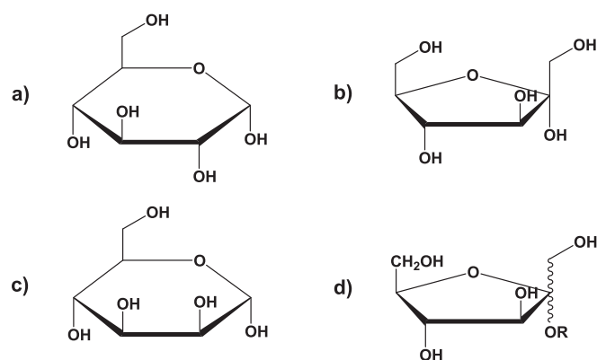
Fig. 2. The chemical structures of: (a) α-D-glucose, (b) α-D-fructose, in its furanose form, (c) α-D-mannose and (d) alkyl fructofuranoside (either α or β form) where R = CH 3 – for a reaction carried out in methanol and CH 3 –CH 2 – for a reaction carried out in ethanol.
