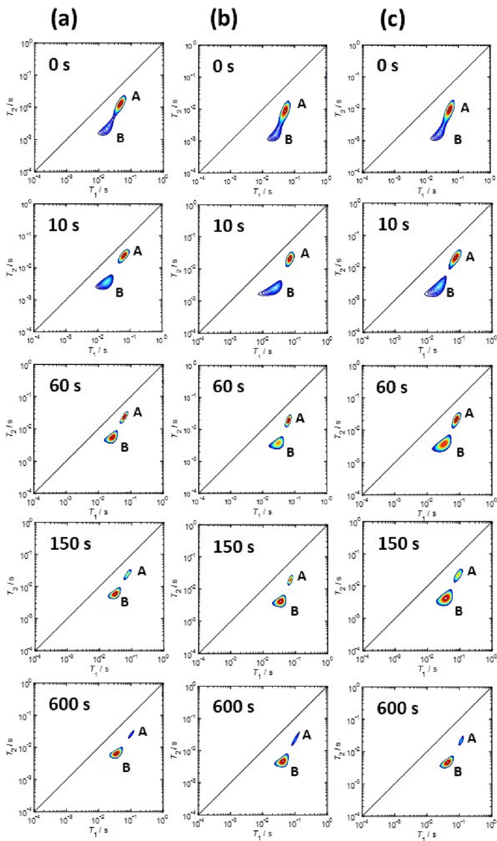
Fig. 6. T_1 - T_2 relaxation correlation plots for ethanol being displaced by water within the pores of (a) HY, (b) Ga/Y and (c) Sn/Y at the displacement time intervals of 0 s, 10 s, 60 s, 150 s and 600 s. A and B represent the aliphatic peak of the alcohol (ethanol) and the OH/water peak, respectively.
