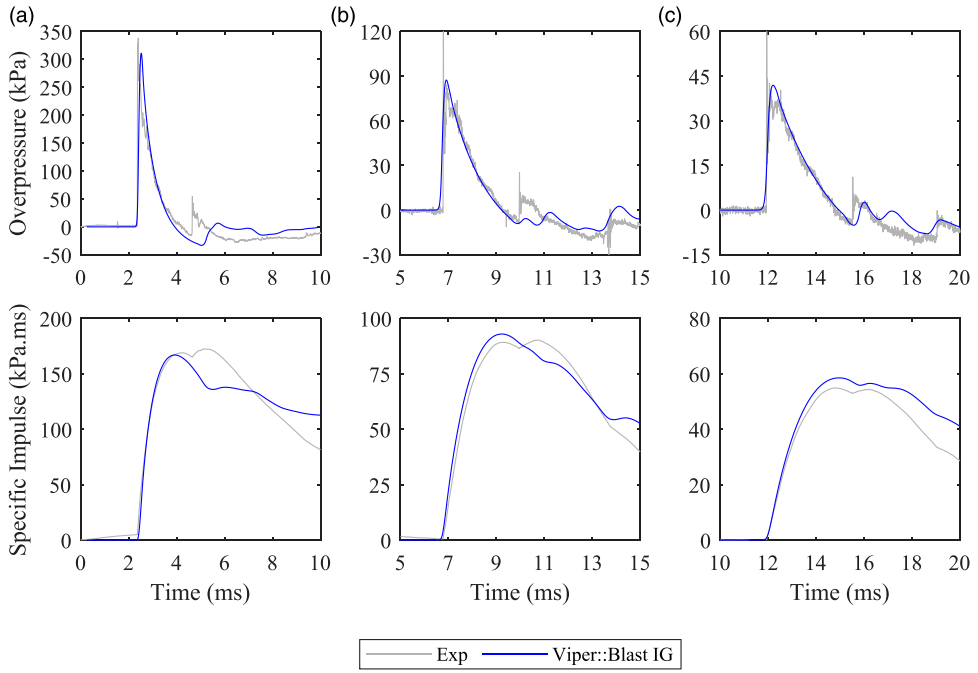
Figure 5. PE4 overpressure-time histories for various PE4 hemispherical charge sizes and stand-offs. (a) 2m 250 g. (b) 4m 350 g. (c) 6m 350 g. Time scales are adjusted so that the arrival times of the Viper models match the experiments.
