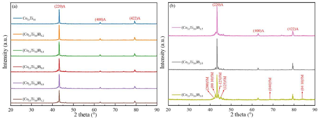
Fig. 3. XRD patterns of (\text{Ni}_{37}\text{Co}_{13}\text{Mn}_{34}\text{Ti}_{16})_{100-x}\text{B}_x ( x = 0\sim 3 ) alloys at RT.
