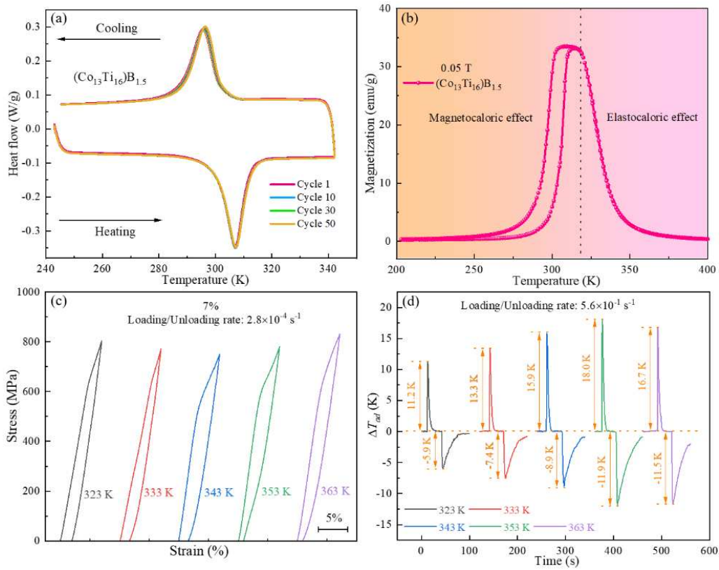
Fig. 12. (a) DSC curves during thermal cycling across martensitic transformation for (\text{Co}_{13}\text{Ti}_{16})\text{B}_{1.5} alloy. (b) M-T curve on heating and cooling under 0.05 T field. (c) Compressive superelastic responses at various temperatures. (d) Time dependence of \Delta T_{ad} on loading/unloading measured at various temperatures.
