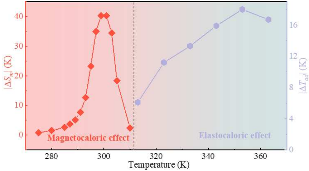
Fig. 13. Temperature dependence of combined caloric effect for (\text{Co}_{13}\text{Ti}_{16})\text{B}_{1.5} alloy.
