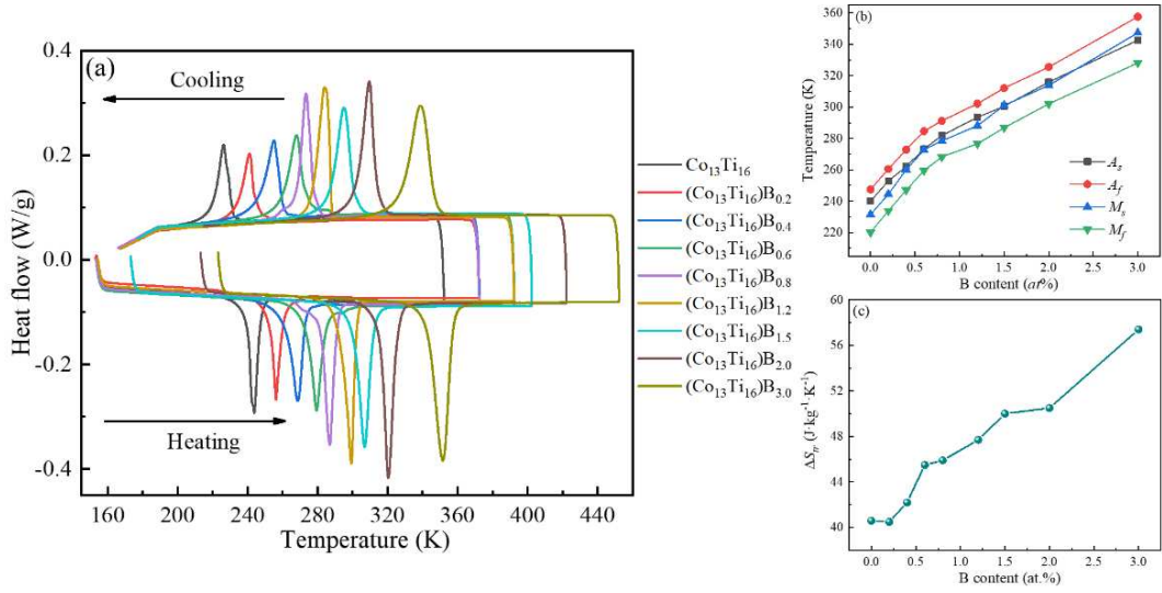
Fig. 1. (a) DSC curves of the martensitic transformation for (\text{Ni}_{37}\text{Co}_{13}\text{Mn}_{34}\text{Ti}_{16})_{100-x}\text{B}_x alloys; (b) and (c) show the reversible martensitic transformation temperature ( M_s , M_f , A_s , and A_f ) and the transformation entropy change \Delta S_{tr} , respectively, as a function of B content.
