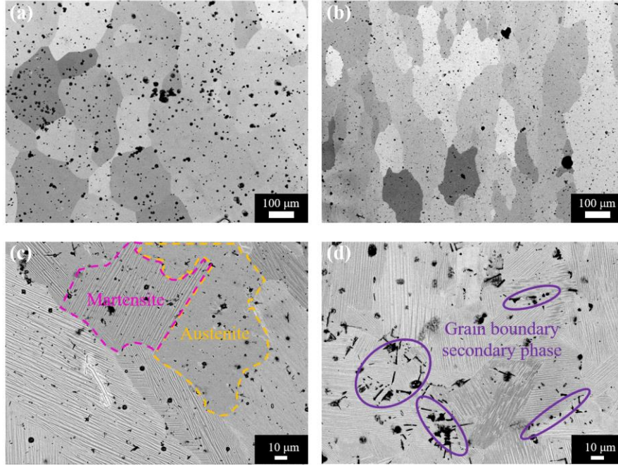
Fig. 6. BSE images of \text{Co}_{13}\text{Ti}_{16} , (\text{Co}_{13}\text{Ti}_{16})\text{B}_{0.8} , (\text{Co}_{13}\text{Ti}_{16})\text{B}_{1.2} , and (\text{Co}_{13}\text{Ti}_{16})\text{B}_{3.0} alloys at RT.
