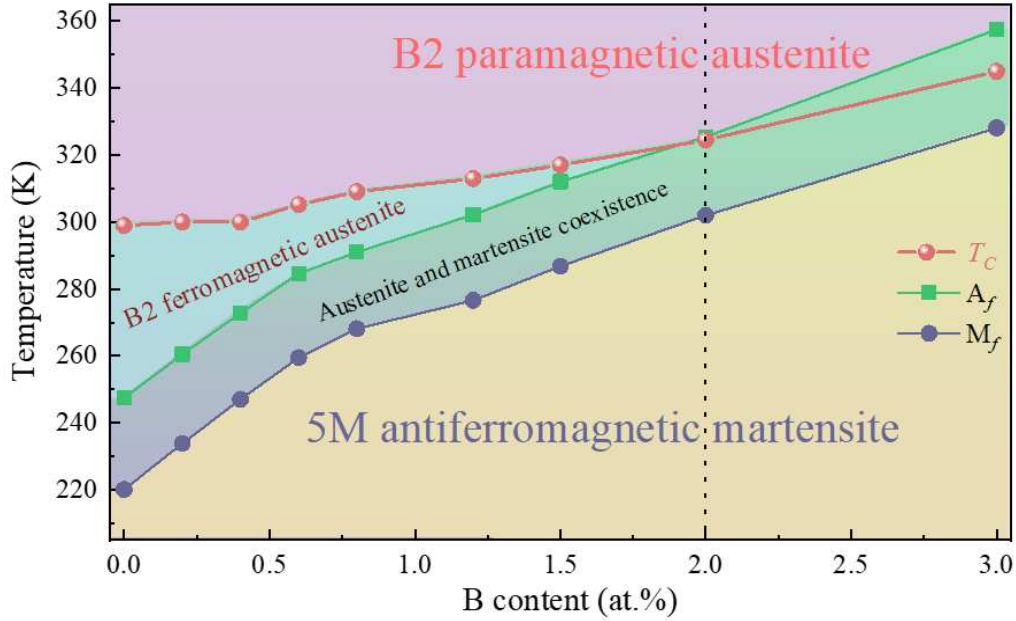
Fig. 10. Magnetic and structural phase diagram of (\text{Ni}_{37}\text{Co}_{13}\text{Mn}_{34}\text{Ti}_{16})_{100-x}\text{B}_x ( x = 0\sim 3 ) alloys.
