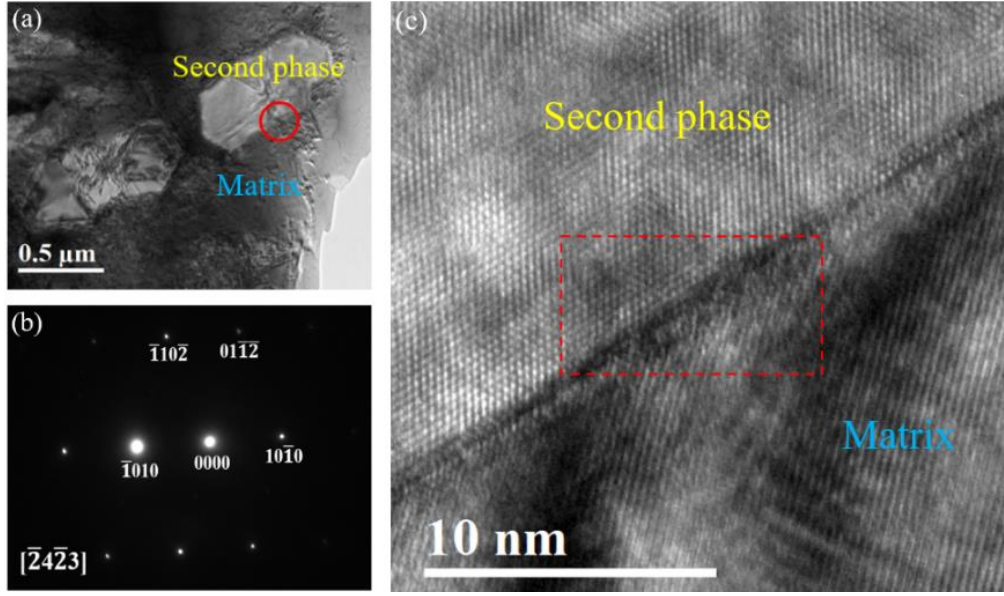
Fig. 7. (a) BFI of the matrix and Ti-rich second phase for (\text{Co}_{13}\text{Ti}_{16})\text{B}_{1.5} alloy. (b) Selected area electron diffraction patterns of Ti-rich second phase. (c) High-resolution TEM image at the interface of the matrix and Ti-rich second phase.
