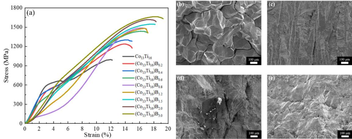
Fig. 5. (a) Stress-strain curves for (\text{Ni}_{37}\text{Co}_{13}\text{Mn}_{34}\text{Ti}_{16})_{100-x}\text{B}_x alloys at 290 K. (b), (c), (d), and (e) SEM micrograph of fractured surface for B0, B0.8, B1.5, and B3 alloys at 298 K.
