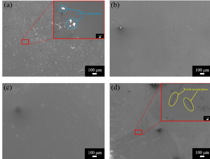
Fig. 2. Second electron images of \text{Co}_{13}\text{Ti}_{16} , (\text{Co}_{13}\text{Ti}_{16})\text{B}_{0.8} , (\text{Co}_{13}\text{Ti}_{16})\text{B}_{1.5} , and (\text{Co}_{13}\text{Ti}_{16})\text{B}_{3.0} alloys at RT.
