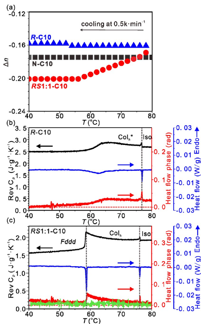
Figure 8. (a) Linear birefringence of compounds R-C10, N-C10, and the RS1:1-C10 mixture. (b, c) MDSC traces of (b) R-C10 and (c) RS1:1-C10. In (b, c), the top (black) curve is the reversing heat capacity, the middle (blue) curve is the total heat flow, and the bottom (red) is the phase lag angle of the complex heat capacity. In MDSC experiments, the cooling rate was 0.04 K/min, the modulation amplitude was \pm 0.07 K, and the modulation period was 20 s. The green trace in (c) was recorded with a modulation period of 60 s. Arrows above the curves point to a relevant scale.
