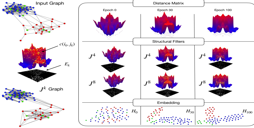
Figure 2: Homophiliation while the jumps and pairwise distances are learned. Top-Left: a heterophilic graph. Center-Left: The current distance matrix \mathcal{D} leads to a tridimensional weight distribution c(i, j) = e^{-d(i, j)} . Yellow points denote the support E_k = \{(i_k, j_k)\} of the filter \mathbf{J}^k . The filter coefficients are given by the weights of the support C_k = \{c(i_k, j_k)\} . Bottom-Left: graph used for aggregation with this filter. In the right panel, we show the weight distribution (top), a couple of filters (middle), and the resulting homophiliation (bottom) for some epochs. In particular, we show \mathbf{H}_0 , \mathbf{H}_{30} and \mathbf{H}_{100} . In each epoch e , all the embeddings \{\mathbf{H}_e^k\} contribute to identifying potential links between scattered nodes with similar labels. If any of these links is wrong, the matrix of pairwise distances \mathcal{D} is updated.
