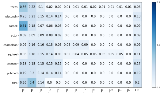
Figure 3: Optimal attention for each jump.
