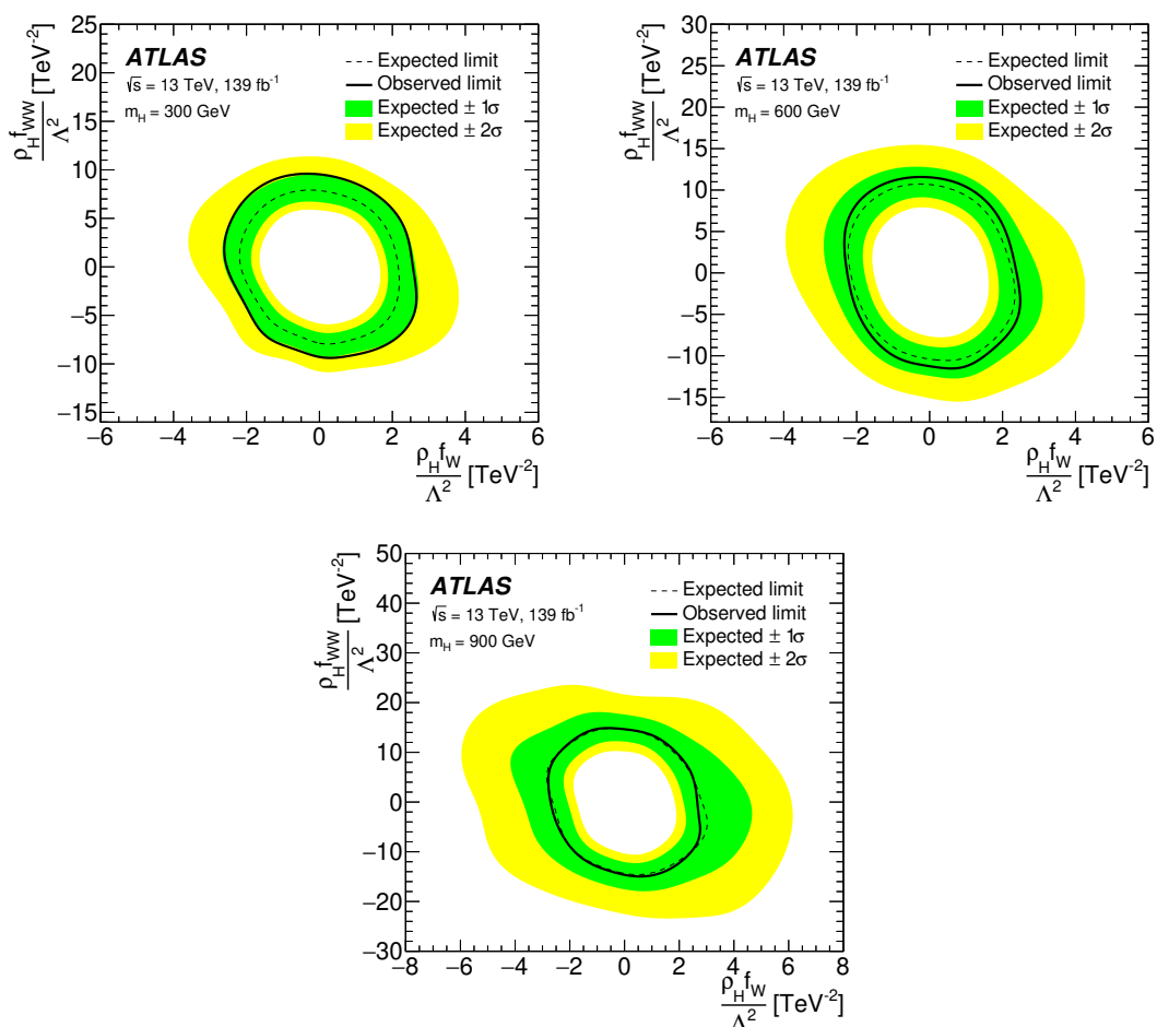
Figure 6. Observed (black solid curve) and expected (black dashed curve) 95% CL upper limits on the production of a heavy Higgs boson as a function of \rho_H f_W/\Lambda^2 and \rho_H f_{WW}/\Lambda^2 for a mass of 300 GeV (top left), 600 GeV (top right) and 900 GeV (bottom). The green (inner) and yellow (outer) bands represent the \pm 1\sigma and \pm 2\sigma uncertainties of the expected limits.
