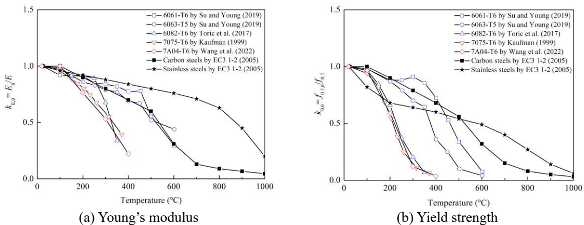
Fig. 1. Comparison of reduction factors for Young's modulus and yield strength of aluminium alloys, carbon steels and stainless steels at elevated temperatures [5-9]
