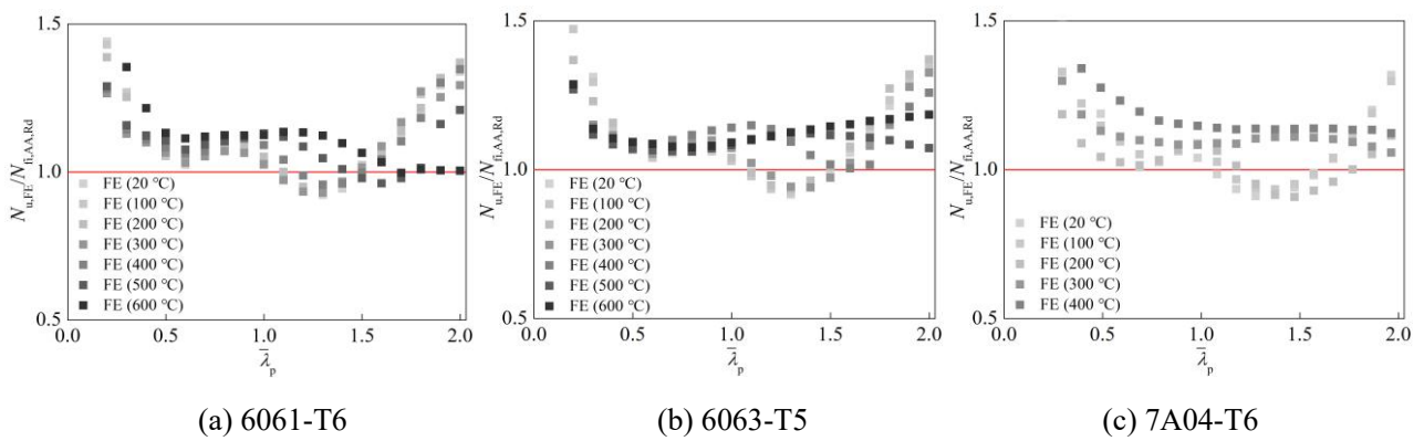
Fig. 14. Comparisons between FE results and resistance predictions according to AA 2015 [25] for outstand plates in compression at different elevated temperatures
