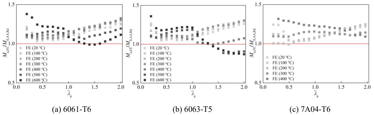
Fig. 13. Comparisons between FE results and resistance predictions according to AA 2015 [25] for internal plates in bending at different elevated temperatures
