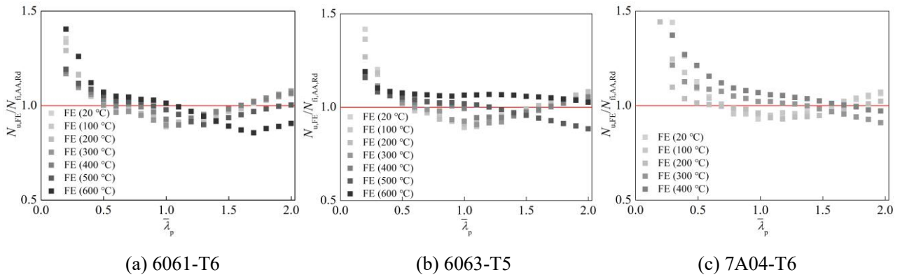
Fig. 12. Comparisons between FE results and resistance predictions according to AA 2015 [25] for internal plates in compression at different elevated temperatures
