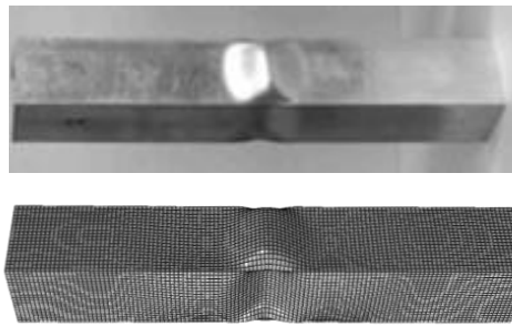
(a) Plates in compression
