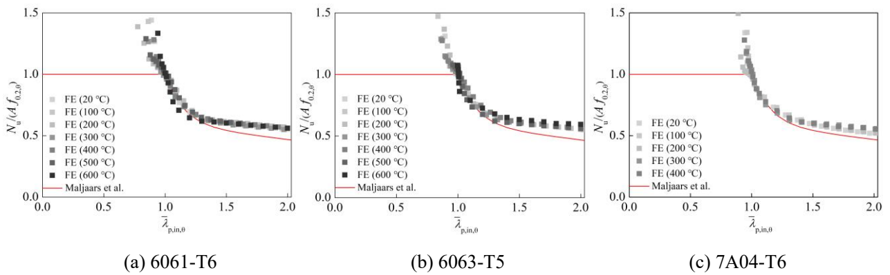
Fig. 19. Comparisons between FE results and resistance predictions according to Maljaars et al. [21] for outstand plates in compression at different elevated temperatures
