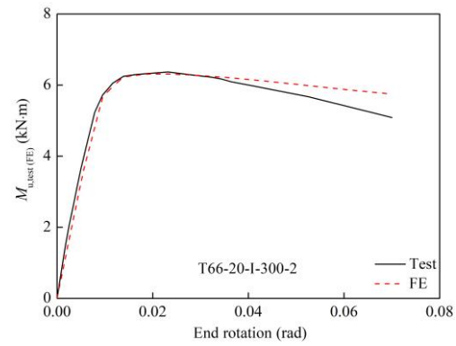
(b) Plates in bending
