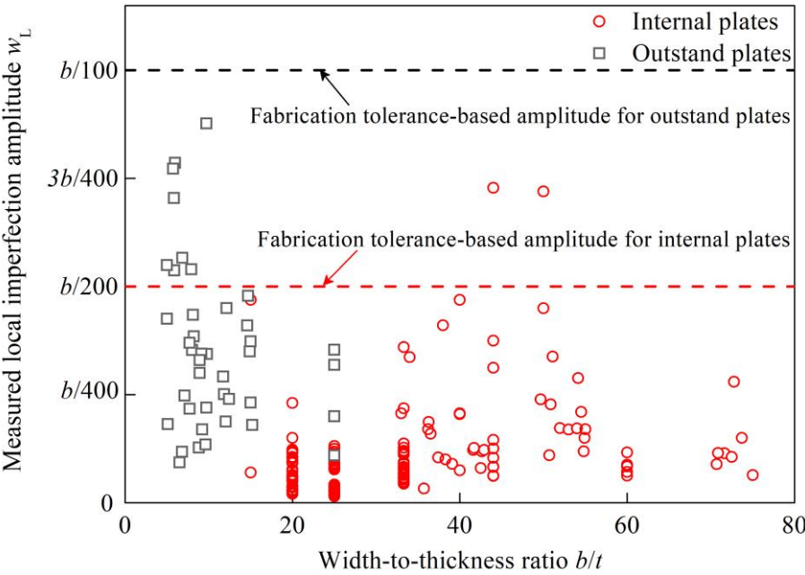
Fig. 3. Summary of measured local imperfection amplitudes of 187 internal and 42 outstand aluminium alloy plates
