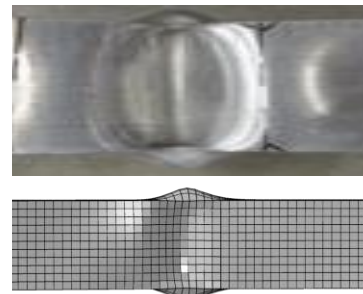
(b) Plates in bending
