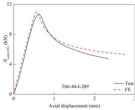
(a) Plates in compression
