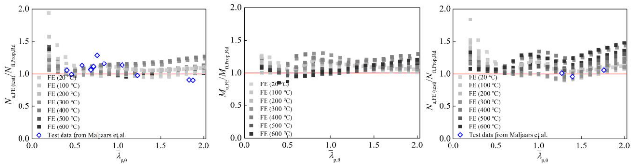
(a) Internal plates in compression (b) Internal plates in bending (c) Outstand plates in compression
