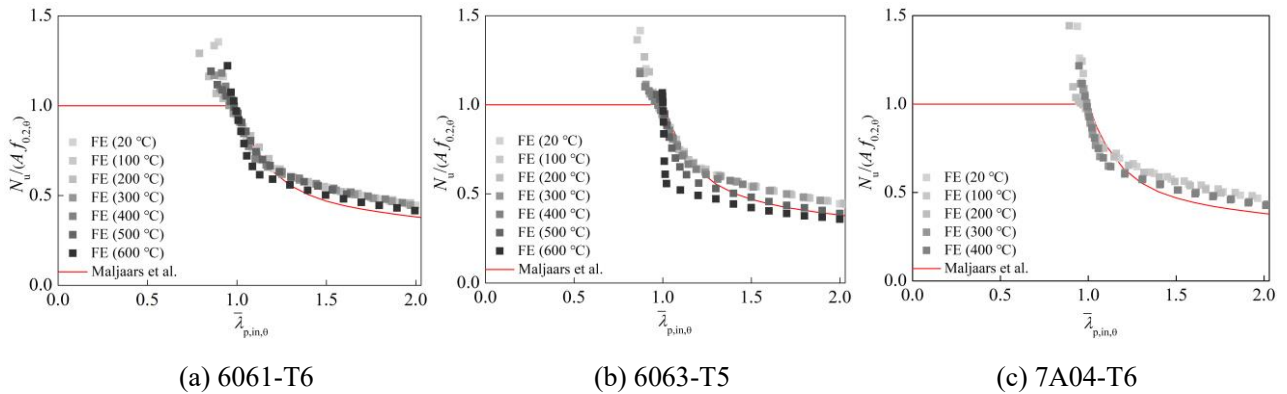
Fig. 18. Comparisons between FE results and resistance predictions according to Maljaars et al. [21] for internal plates in compression at different elevated temperatures
