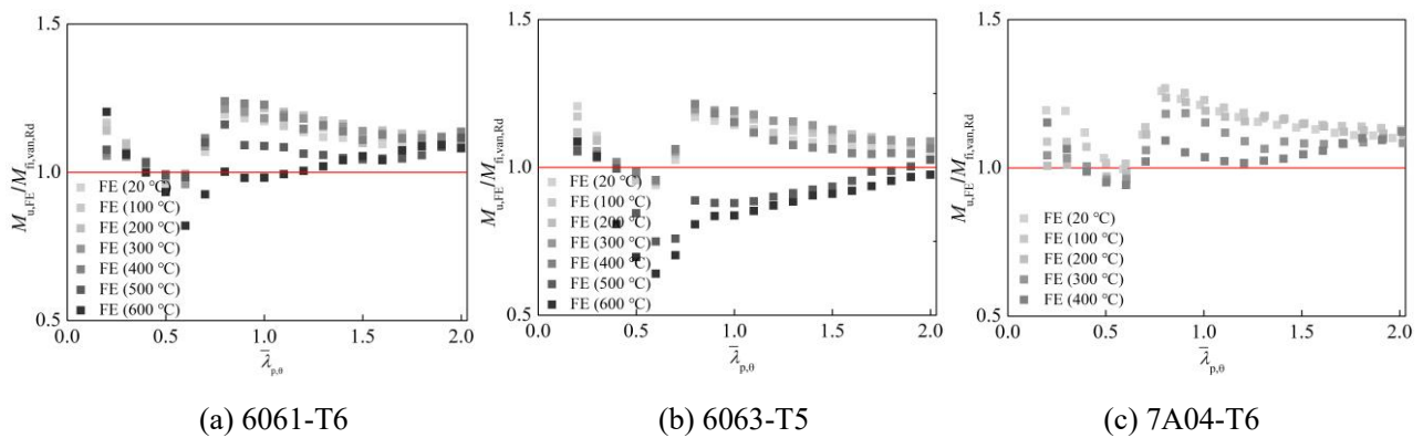
Fig. 20. Comparisons between FE results and resistance predictions according to van der Meulen [22] for internal plates in bending at different elevated temperatures
