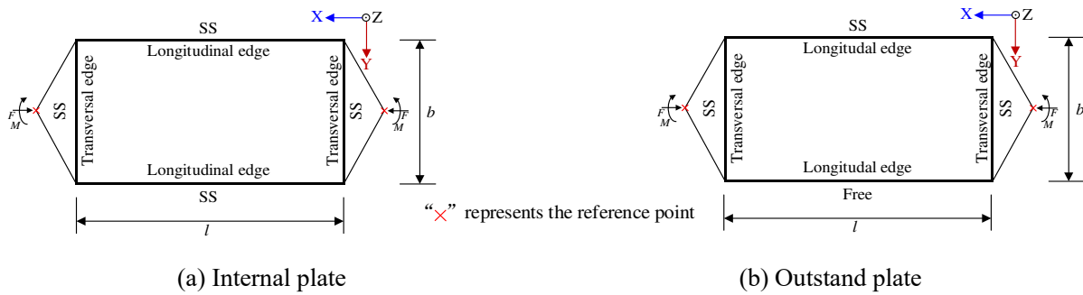
Fig. 2. Boundary conditions of internal and outstand plates
