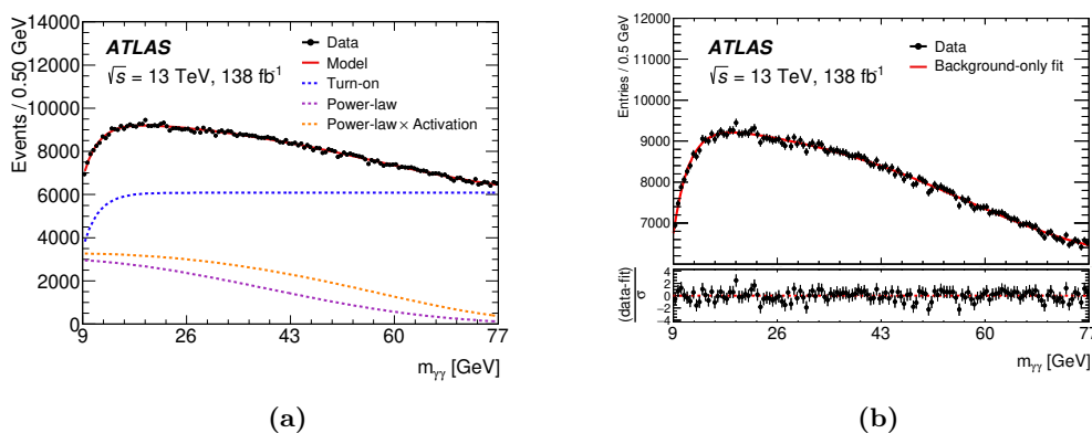
Figure 5. (a) Distribution of the diphoton invariant mass for all events passing the analysis selections in the full Run 2 dataset with the background-only fit superimposed. The functional form is decomposed into the different pieces described in detail in section 6.1. (b) Vertically enlarged version of figure 5a. The normalized residuals between the data and the fit are shown in the bottom panel.
