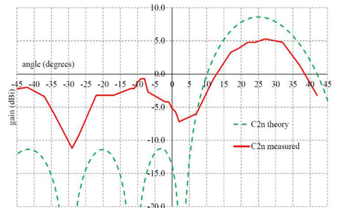
FIGURE 27. C2n beam ACG for C2n steered to +25 degrees.
