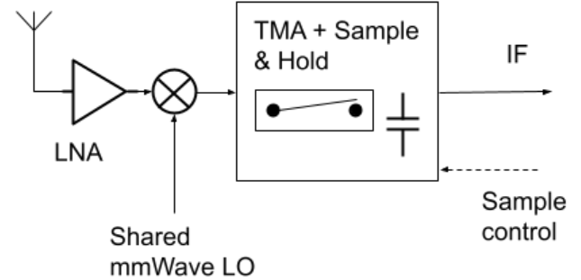
FIGURE 29. Prototype mmWave STMA cell with mixer-first down conversion to intermediate IF due to limited switch RF BW.
