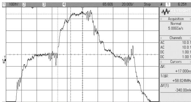
FIGURE 15. Example time domain capture of 3 cycles of T_s sampler capacitor C22 voltage, showing 17 ns rise and 33 ns hold times in a 50 ns sampling interval.
