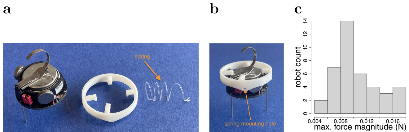
Fig. 5 | Overview of the module of the Kilobot Soft Robot. a Up to four helical springs can be connected to the Kilobot through a 3-D printed circllet. b Kilobot equipped with the circllet. The circllet is firmly attached to the Kilobot (i.e. the latter can not rotate within the circllet). Four springs are attached at fixed mounting holes,
