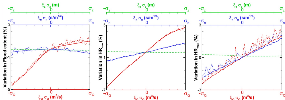
Figure 5. Torrential flooding over a rough river valley (Section 2.5.2). Centerline plots of the projections from the D -dimensional response surfaces for Flood Extent, \text{HR}_{\text{ave}} , and \text{HR}_{\text{max}} , showing their variations in each uncertainty dimension for the case with D = 2 (solid lines) and the case with D = 3 (dotted lines).
