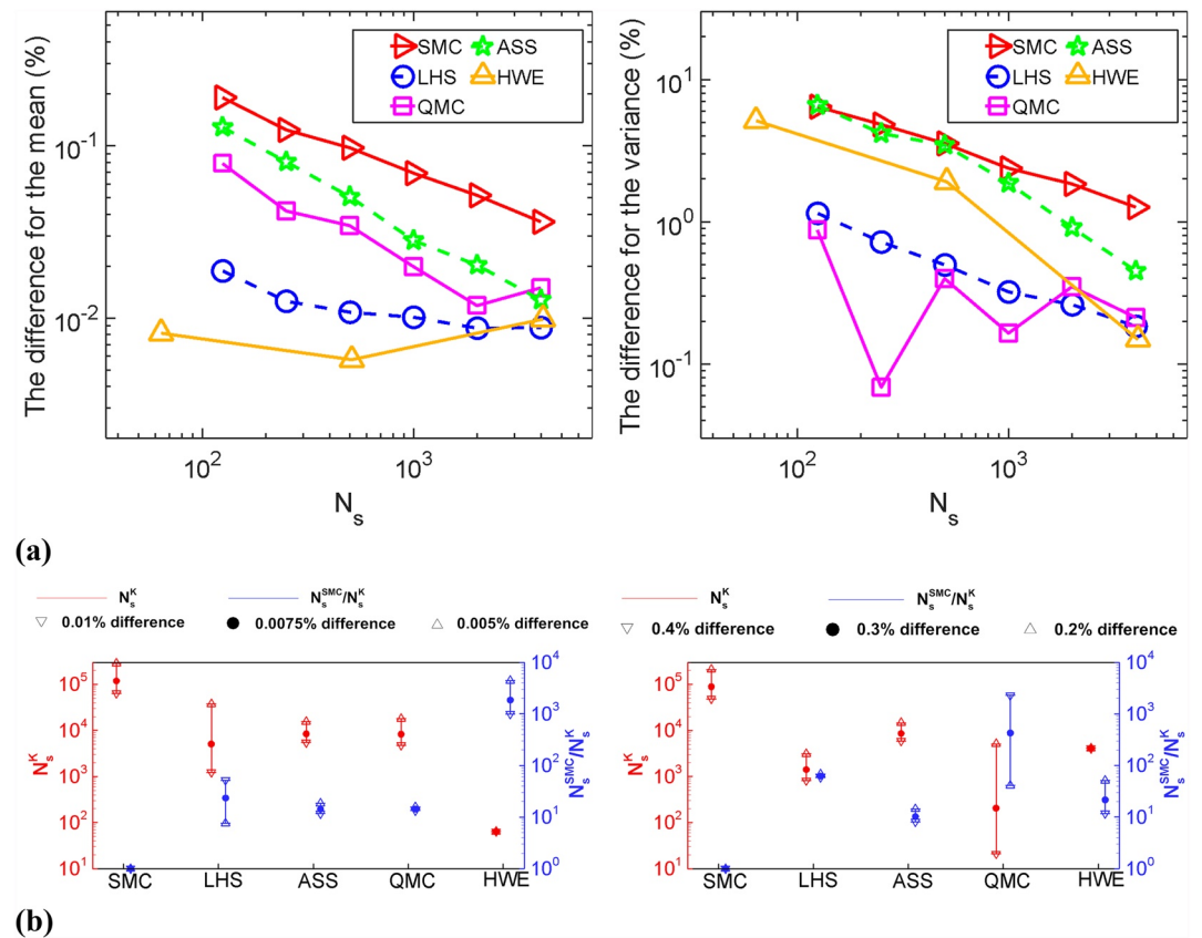
Figure A3. Rapidly propagating flood over a smooth terrain (Section 2.5.1). Panel (a) shows the order of convergence per UQ method K ( K = \text{SMC}, \text{QMC}, \text{HWE}, \text{LHS}, \text{and ASS} ) calculated for HR_{\max} based on the difference in the standard errors of the mean (left) and the variance (right); and, panel (b) shows the N_s^K and relative-to-SMC speedup ratio for HR_{\max} to meet the target difference: of 0.0075\% \pm 0.0025\% based on the standard error of the mean (left), and of 0.3\% \pm 0.1\% based on the standard error of the variance (right).
