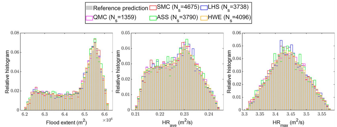
Figure 14. Torrential flooding over a rough river valley (Section 2.5.2). Relative histograms with N_{\text{bins}} = 40 for Flood Extent (left), HR_{\text{ave}} (middle) and HR_{\text{max}} (right) per uncertainty quantification method K ( K = standard Monte Carlo, QMC, Haar-wavelet expansion, Latin hypercube sampling, and adaptive stratified sampling) for the N_s^K identified for the sub-case with D = 2 (Section 3.1.1).
