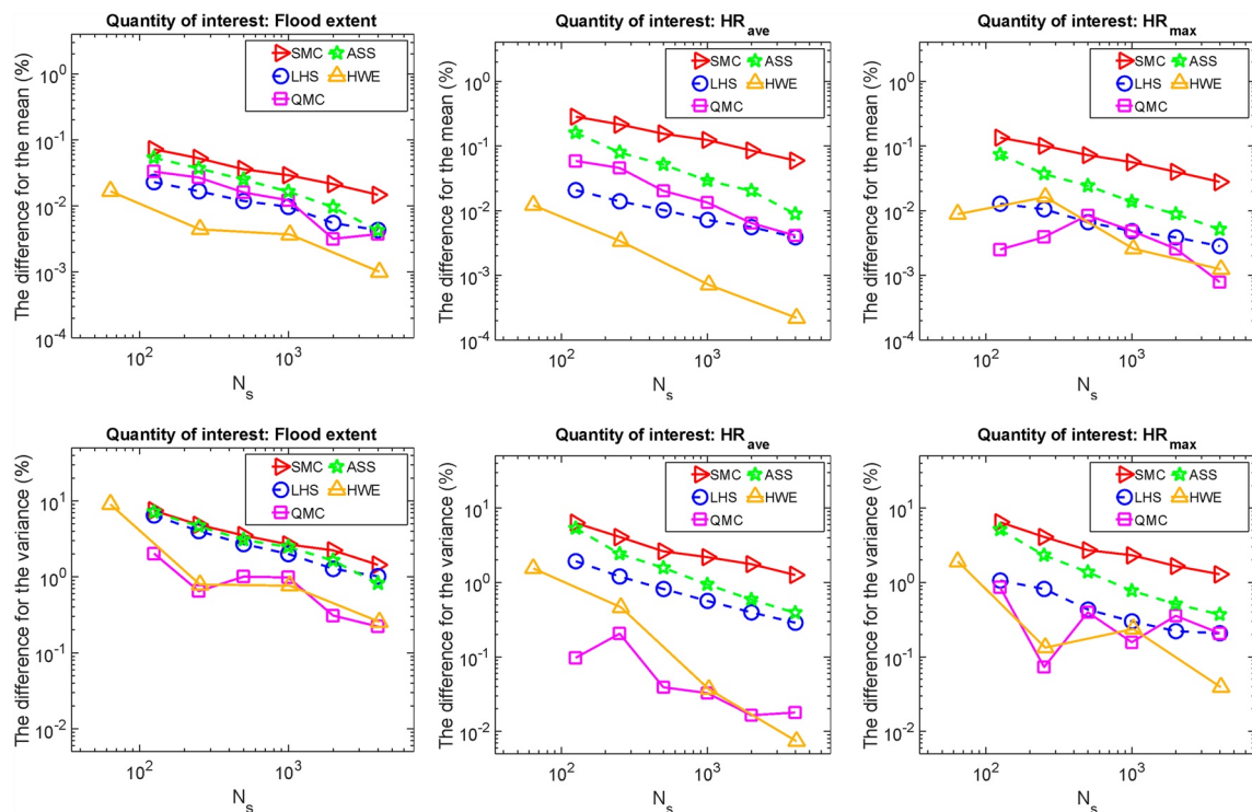
Figure A1. Rapidly propagating flood over a smooth terrain (Section 2.5.1). Order of convergence per uncertainty quantification method K ( K = \text{standard Monte Carlo} , \text{QMC} , \text{Haar-wavelet expansion} , \text{Latin hypercube sampling} , and \text{adaptive stratified sampling} ) calculated for Flood Extent, \text{HR}_{\text{ave}} , and \text{HR}_{\text{max}} based on the difference in the mean (upper panel) and variance (lower panel).
