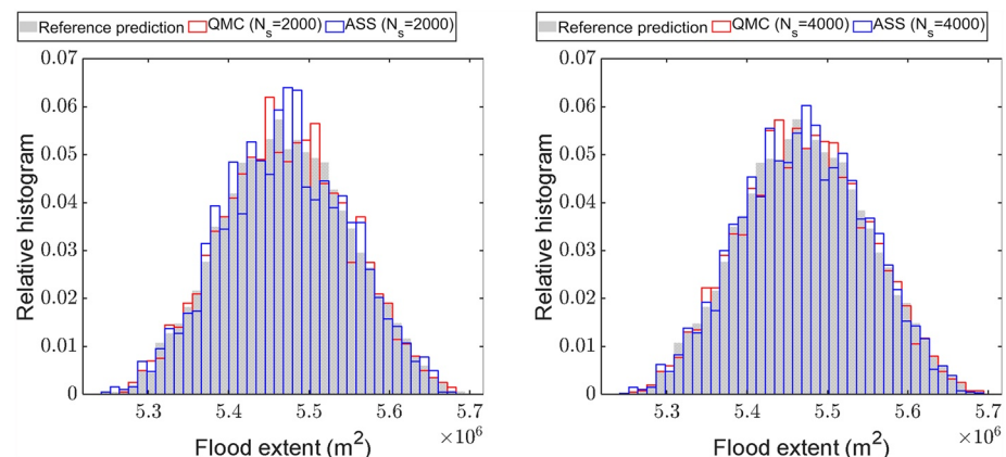
Figure 16. Carlisle 2005 flooding (Section 2.5.3). Relative Flood Extent histograms (using N_{\text{bins}} = 40 ) per uncertainty quantification method K ( K = \text{QMC} and adaptive stratified sampling) for N_s^K = 2,000 (left) and 4,000 (right).
