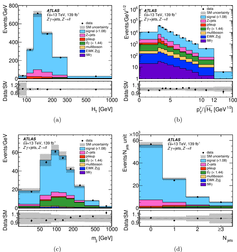
Figure 4. The measured (a) H_T , (b) p_T^\gamma/\sqrt{H_T} , (c) m_{jj} , and (d) N_{jets} distribution (dots) in the signal region. The error bars represent the data statistical uncertainty; for most of the points, the error bars are smaller than the marker size and, thus, not visible. The MC simulation of the signal from SHERPA 2.2.11 (blue histograms) and various backgrounds are also included. The signal and background distributions are stacked to produce the figures. The variable bin width is taken into account in the vertical scale. The lower part of each figure shows the ratio of the data to the expected total SM distribution. The hatched band represents the statistical and systematic uncertainties on the SM background yields added in quadrature, excluding theory uncertainties of the signal.
