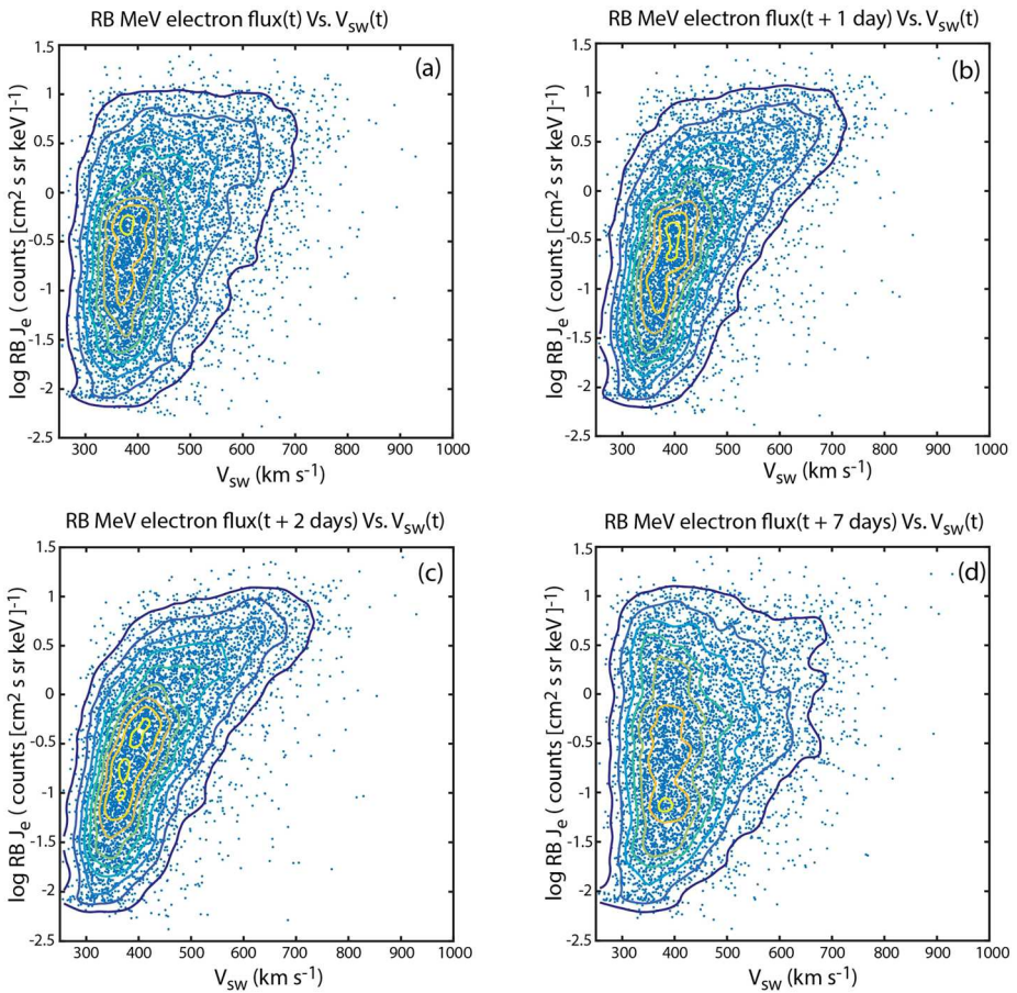
Fig. 11 (Fig. 1 from Wing et al. 2016) Scatter plots of \log J_{e,\text{GEO}}(t + \tau) vs. V_{\text{sw}}(t) for \tau = 0, 1, 2, and 7 days in panels (a), (b), (c), and (d), respectively. The data points are overlain with density contours showing the nonlinear trends. The panels show that J_{e,\text{GEO}} has dependence on V_{\text{sw}} for \tau = 0, 1, and 2 days and the dependence is strongest for \tau = 2 days. (d) At large \tau , e.g., \tau = 7 day, J_{e,\text{GEO}} dependence on V_{\text{sw}} is very weak. The triangle distribution (Reeves et al. 2011) can be seen in panels (a), (b), and (c). This is essentially the same as Fig. 10 in Reeves et al. (2011), except that no density contours are drawn and Fig. 9d plots \tau = 7 days instead of \tau = 3 days
