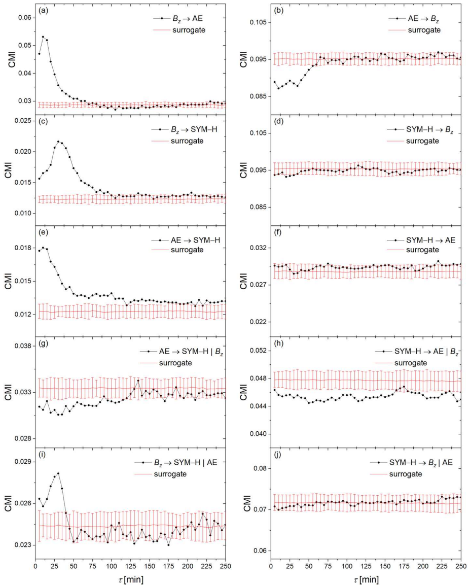
Fig. 1 (Fig. 3 from Manshour et al. 2021) The coupling directions of (a) B_z \rightarrow AE , (b) AE \rightarrow B_z , (c) B_z \rightarrow SYM - H , (d) SYM - H \rightarrow B_z , (e) AE \rightarrow SYM - H , and (f) SYM - H \rightarrow AE . (g) and (h) are the coupling directions similar to (e) and (f), by taking B_z as the common driver. Also (i) and (j) are the coupling directions similar to (c) and (d), by taking AE as the common driver. The red lines and error bars present mean and \pm 2 standard deviations of CMI for a set of 100 circular time-shifted surrogates
