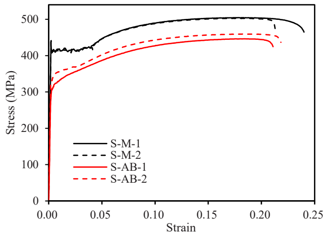
Fig. 6. Engineering stress-strain curves of machined (M) and as-built (AB) WAAM coupons.
