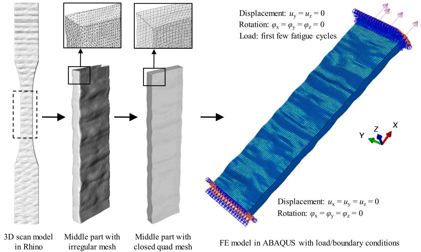
Fig. 11. Development of a finite element model from a 3D scan model.
