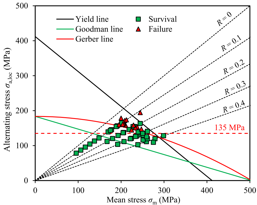
Fig. 15. Assessment of fatigue test results in a CLD based on local stresses.
