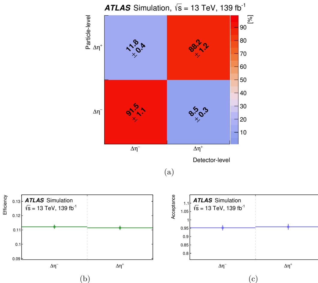
Figure 6. (a) The migration matrix and (b,c) the efficiency/acceptance corrections that are used as input for the unfolding of SR-2b-low N_{\text{jets}} . The matrices are normalised such that the sum of any given row is 100%, although small differences may be present due to rounding. The error bars of the efficiency/acceptance correction terms represent the MC statistical uncertainties per bin based on the nominal t\bar{t}W SHERPA sample.
