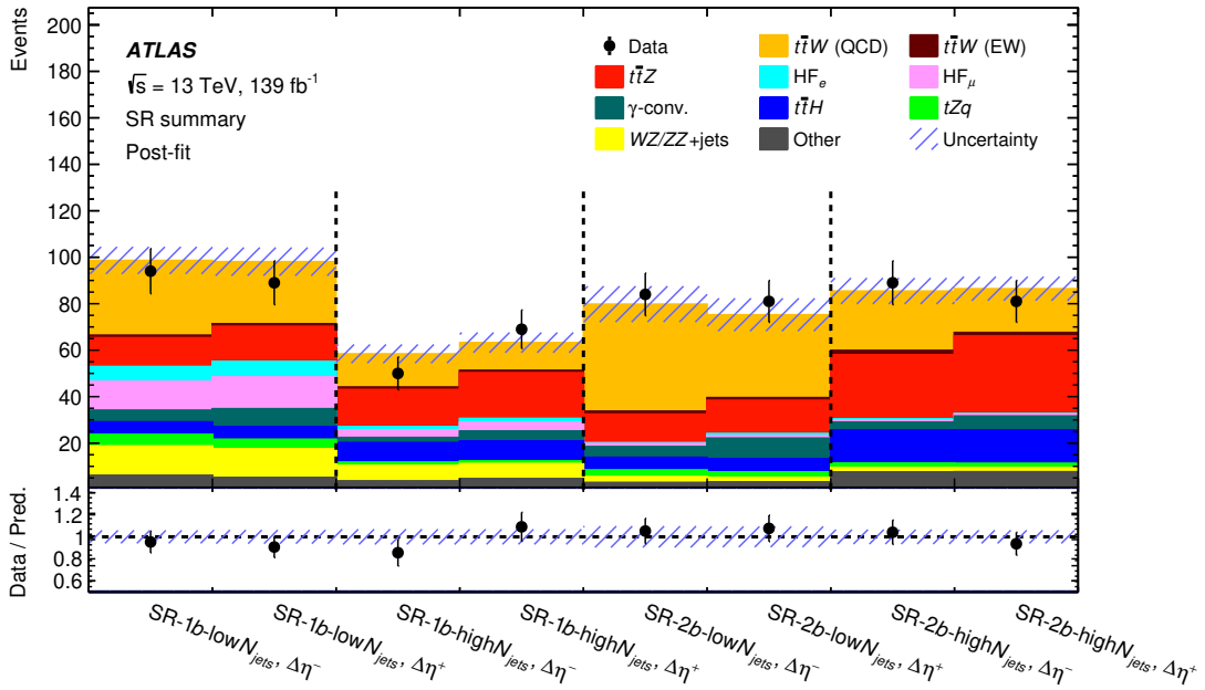
Figure 2. Comparison between data and the post-fit predictions for \Delta\eta_{\text{BDT}}^{\ell} \leq 0 ( \Delta\eta^{-} ) and \Delta\eta_{\text{BDT}}^{\ell} > 0 ( \Delta\eta^{+} ) in the four SRs. The error band includes the total uncertainties of the post-fit predictions, with the exception of the \Delta\eta^{\pm} CR-dependency uncertainty. The ratio of the data to the total post-fit predictions is shown in the lower panel.
