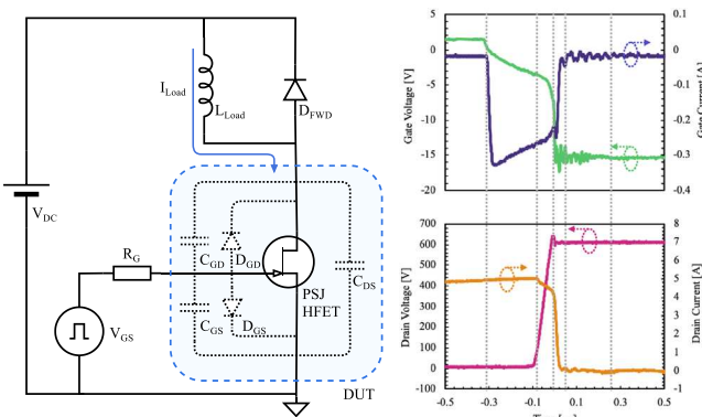
Fig. 6. Experimental setup and the typical turn-off switching waveforms.
