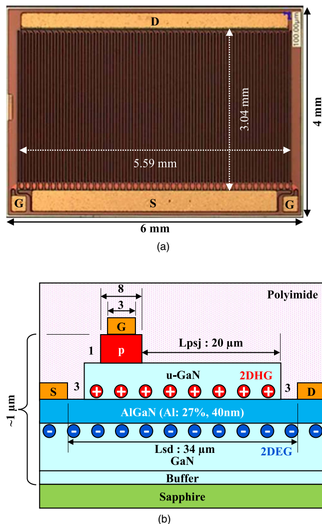
Fig. 1. (a) Top view of a 1.2 kV GaN PSJ HFET chip and (b) a cross-sectional view of the device structure. Gate, drain and source are marked as G, D and S, respectively.
