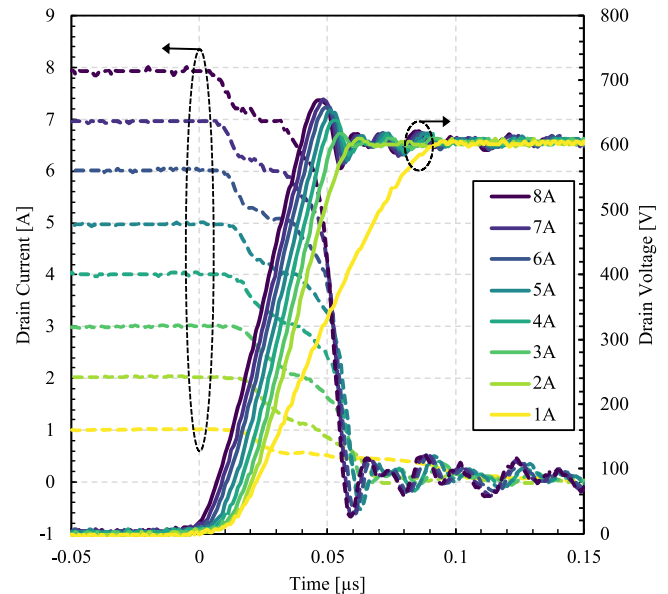
Fig. 12. Measured turn-off switching waveforms of the GaN PSJ HFET at different load currents. The supply voltage is constant at 600 V.
