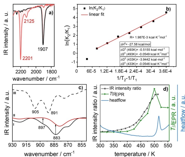
Figure 5. a) FT-IR spectra of ( o -1) 2 in solid-state upon heating from room temperature (black line) to 240 °C (red line). b) Van't Hoff fitting for the dimerization process in the solid-state from the absorbances of the 2201 and 1907 (bands) with universal gas constant R . c) Theoretical infrared spectrum at the B3LYP/6-31G** level of the dimer from the crystalline structures (III), the experimental IR spectra at room temperature (I) and upon heating to 240 °C (II). d) Comparison of the intensity ratio of the increasing CN band at 2201 cm -1 , DSC plot (N 2 ) and TII/EPR vs. temperature.
