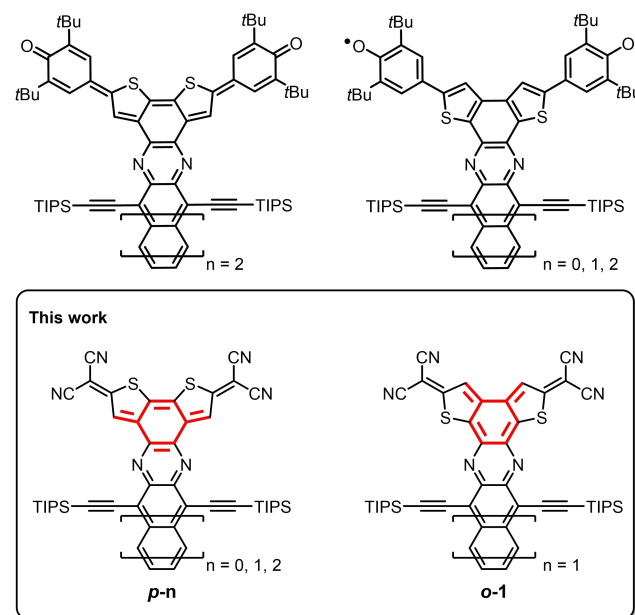
Figure 2. Top: Previously reported phenoxyl-based azaacene quinoids/diradicals. [18d] Bottom: Chemical structures of the studied compounds herein. p-n and o-1 include para - and ortho -xylylene substructures between the tetracyanated, quinoidal bithiophene segment (marked in red). The quinoidal resonance forms are depicted.
