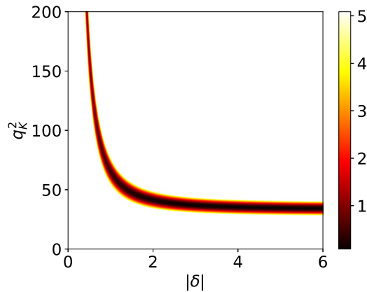
FIG. 27. The \chi^2 plot as a function of the |\delta| and q_K^2 mixing parameters of the 2_2^+ \rightarrow 2_1^+ 197 keV transition in ^{182}\text{Hg} . The \chi^2 value is given by the color scale.
