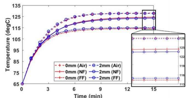
Fig. 3. Maximum winding temperature for the modular ( \text{FG}=2 \text{ mm} ) and non-modular machines ( \text{FG}=0 \text{ mm} ) with different coolants such Air, NF (nanofluid) and FF (ferrofluid).
