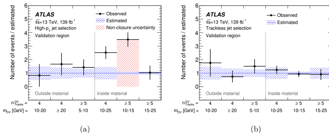
Figure 5. Background estimates relative to expectations for (a) the High- p_T jet selection and (b) the Trackless jet selection showing validation regions with varying n_{Tracks}^{DV} and m_{DV} requirements. Validation regions labeled Outside (Inside) material contain events with a displaced vertex which is accepted (rejected) by the material map veto requirement. The error band dashed with a positive slope includes all systematic uncertainties. The size of the non-closure uncertainty is shown by the band dashed with a negative slope, which is not propagated to the other validation regions in this figure.
